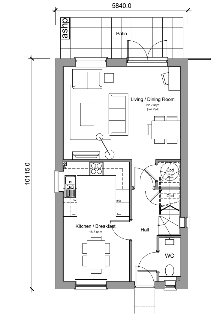
Ground Floor Plan 3-Bedroom 5-Person House 96.78sqm / 1042sqft GIA [to finishes]
