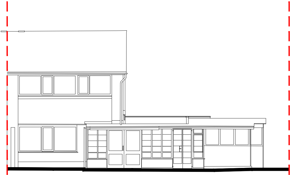
Existing South Elevation - 5 Birkdale Road
