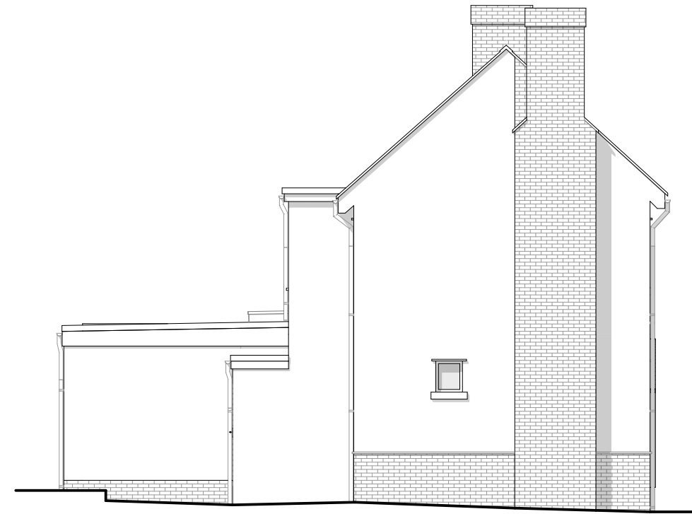
Existing Side (North) Elevation Scale 1:100 @ A3
