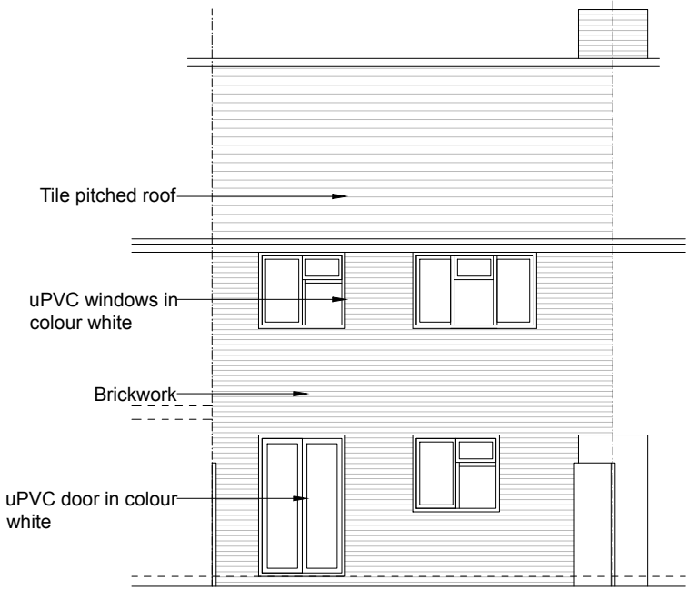
Rear (North) Elevation as existing
