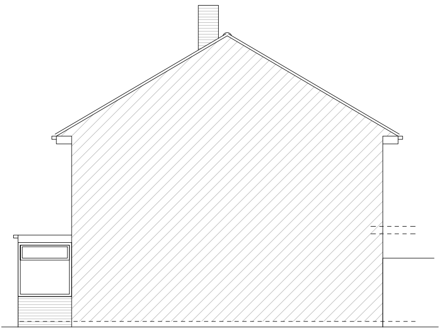
Side (East) Elevation as existing
