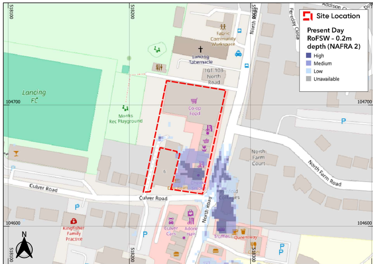
Figure 6: RoFSW Likelihood of Depths Exceeding 0.2m. (Base map and data from OpenStreetMap and OpenStreetMap Foundation (CC-BY-SA). © https://www.openstreetmap.org and contributors. Contains public sector information licensed under the Open Government Licence v3.0)
