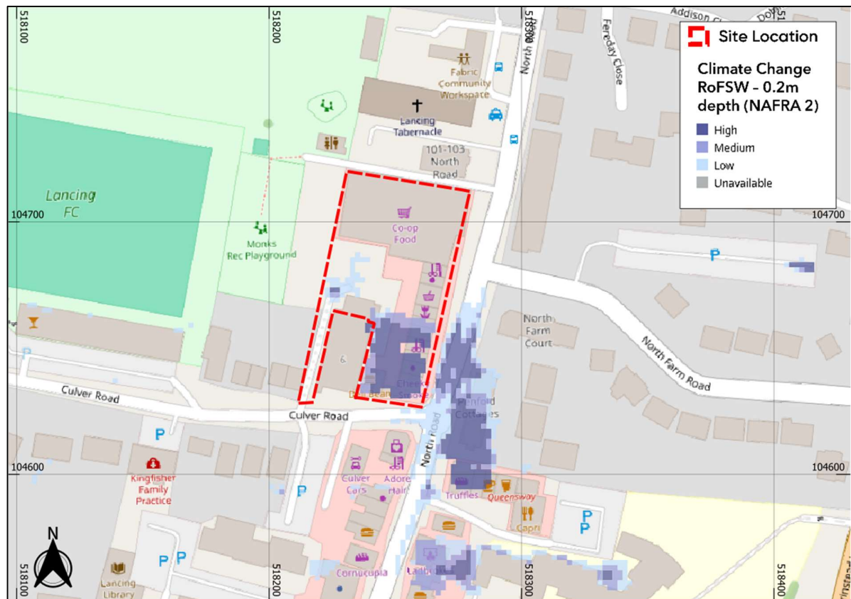
Figure 10: RoFSW Likelihood of Depths Exceeding 0.2m. (Base map and data from OpenStreetMap and OpenStreetMap Foundation (CC-BY-SA). © https://www.openstreetmap.org and contributors. Contains public sector information licensed under the Open Government Licence v3.0)
