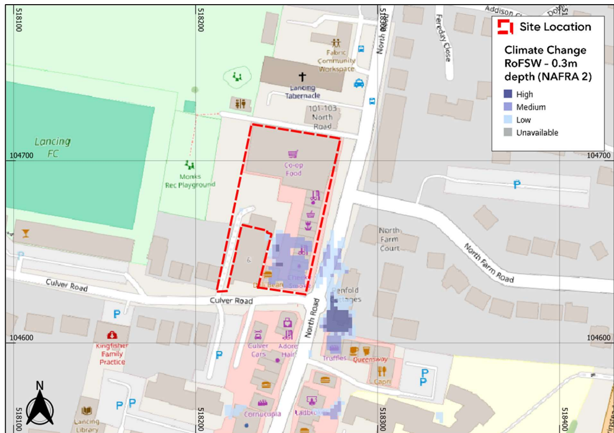
Figure 11: RoFSW Likelihood of Depths Exceeding 0.3m. (Base map and data from OpenStreetMap and OpenStreetMap Foundation (CC-BY-SA). © https://www.openstreetmap.org and contributors. Contains public sector information licensed under the Open Government Licence v3.0)
