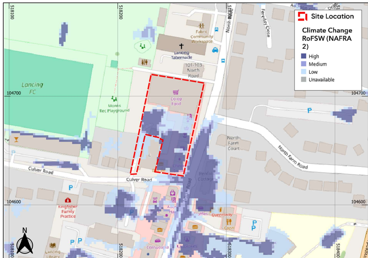
Figure 9: EA Surface Water Flood Risk with Climate Change Mapping. (Base map and data from OpenStreetMap and OpenStreetMap Foundation (CC-BY-SA). © https://www.openstreetmap.org and contributors. Contains public sector information licensed under the Open Government Licence v3.0)
