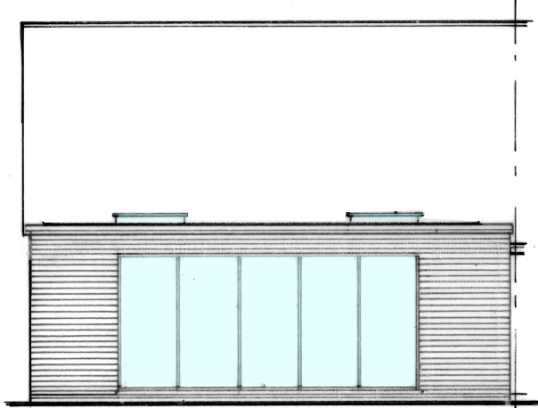
Proposed Rear Elevation ( West) 1:100
