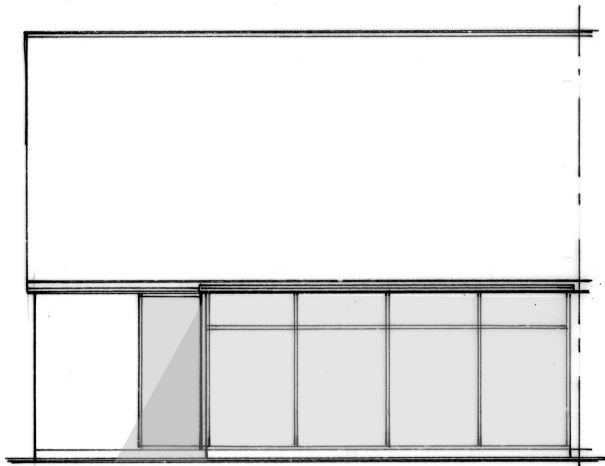
Existing Rear Elevation ( West) 1:100
