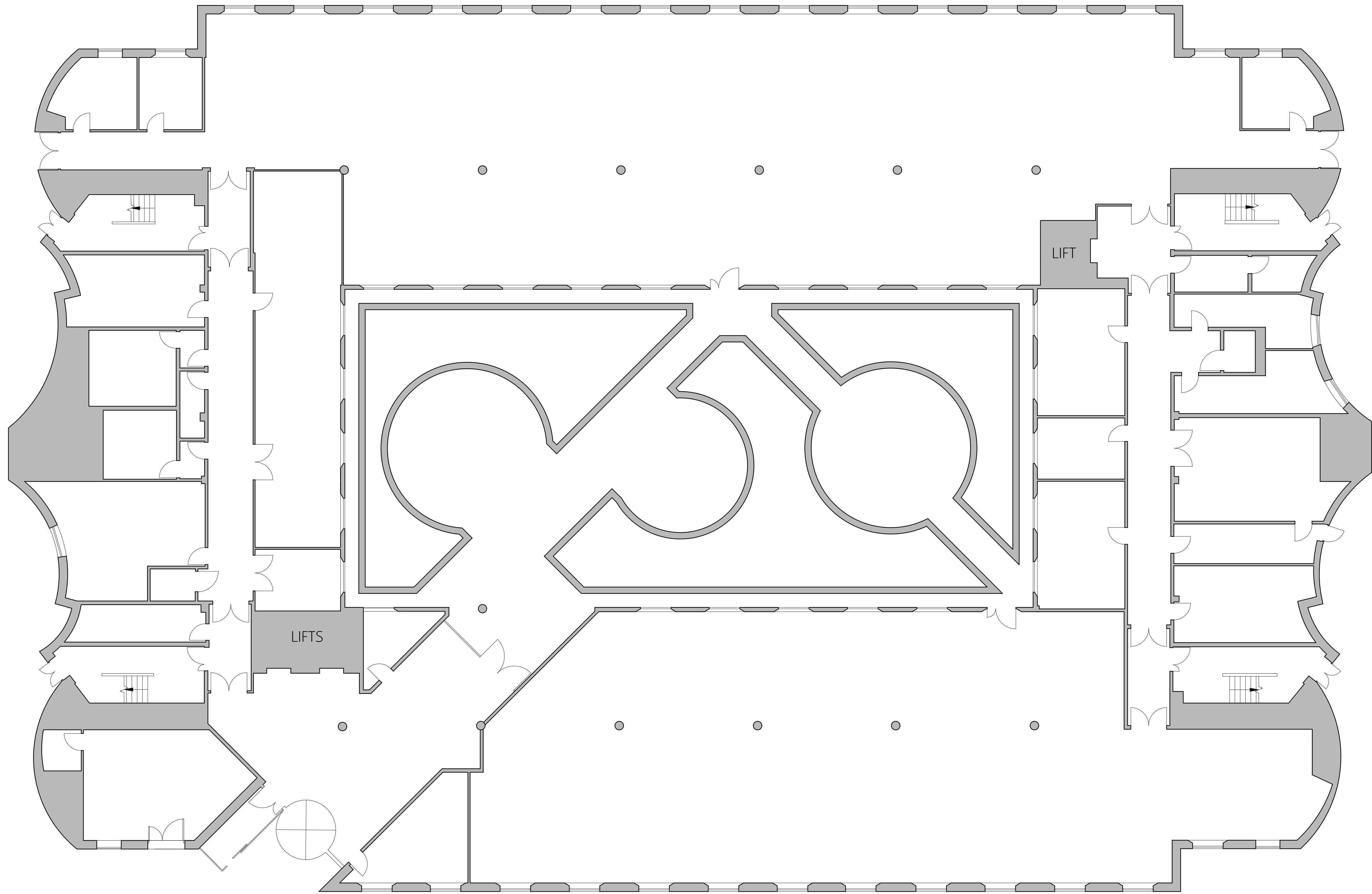
Existing Ground Floor Plan 1:100@A1
