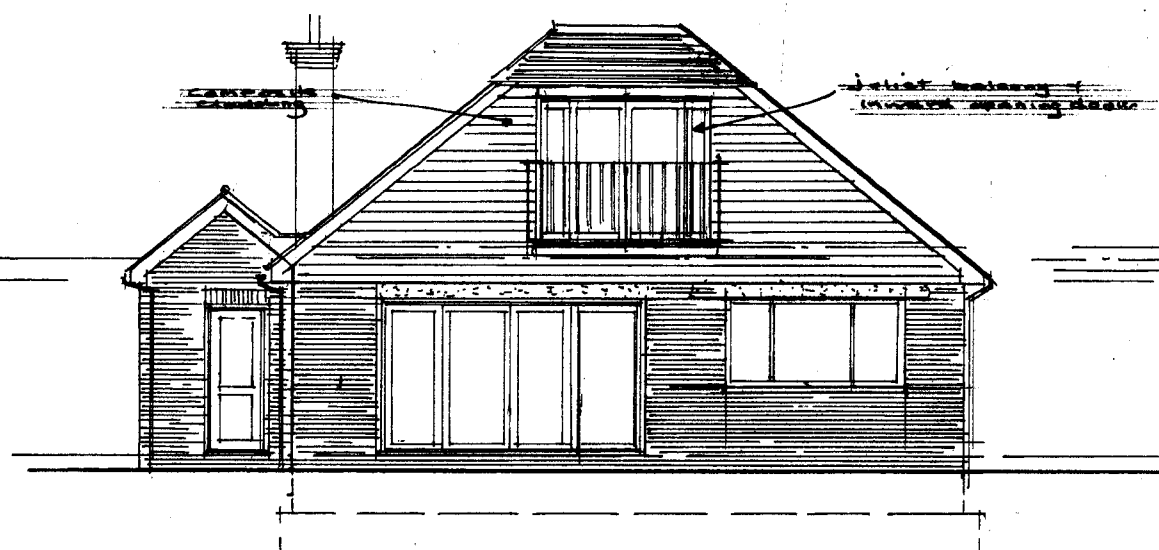
SOUTH ELEVATION
