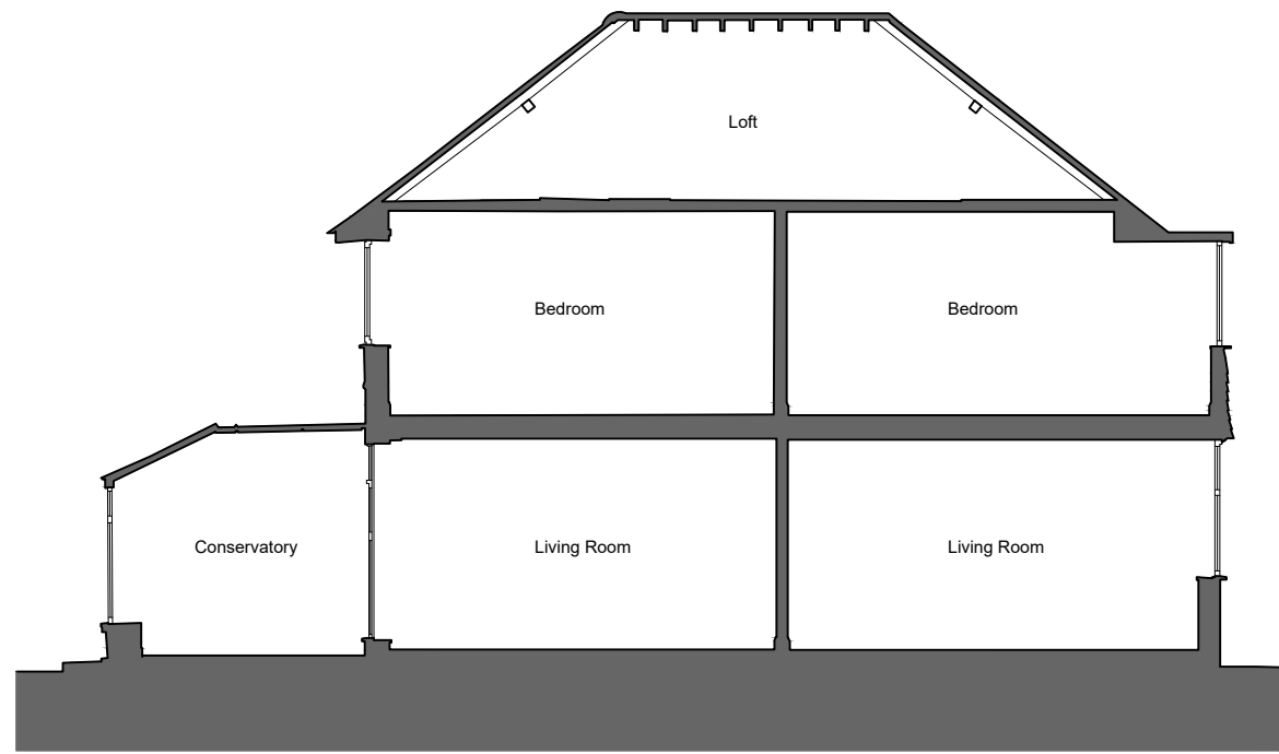
09 | EXISTING SECTION BB 1:100
