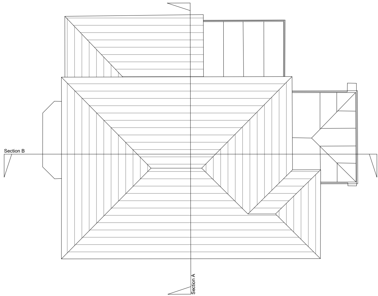
03 | EXISTING ROOF PLAN 1:100
