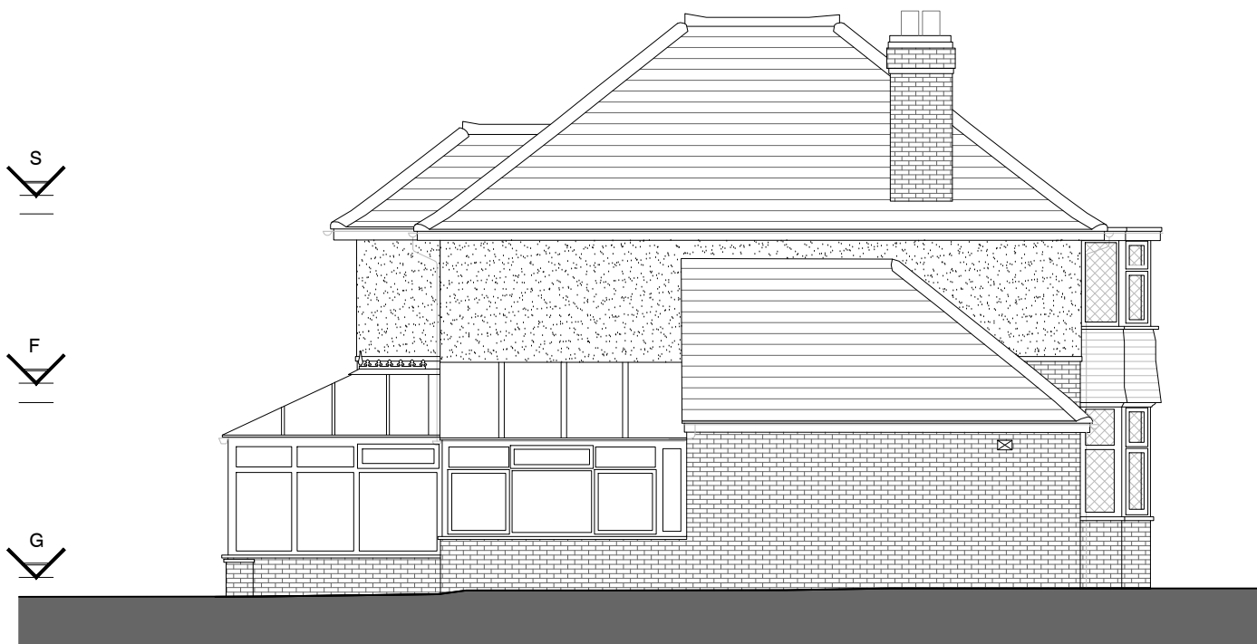
06 | EXISTING SIDE ELEVATION (EAST FACING) 1:100
