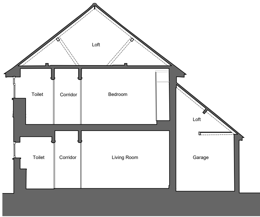
08 | EXISTING SECTION AA 1:100
