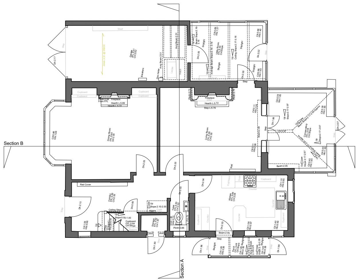
01 | EXISTING GROUND FLOOR PLAN 1:100
