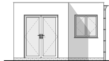
Proposed Front (West) Elevation
