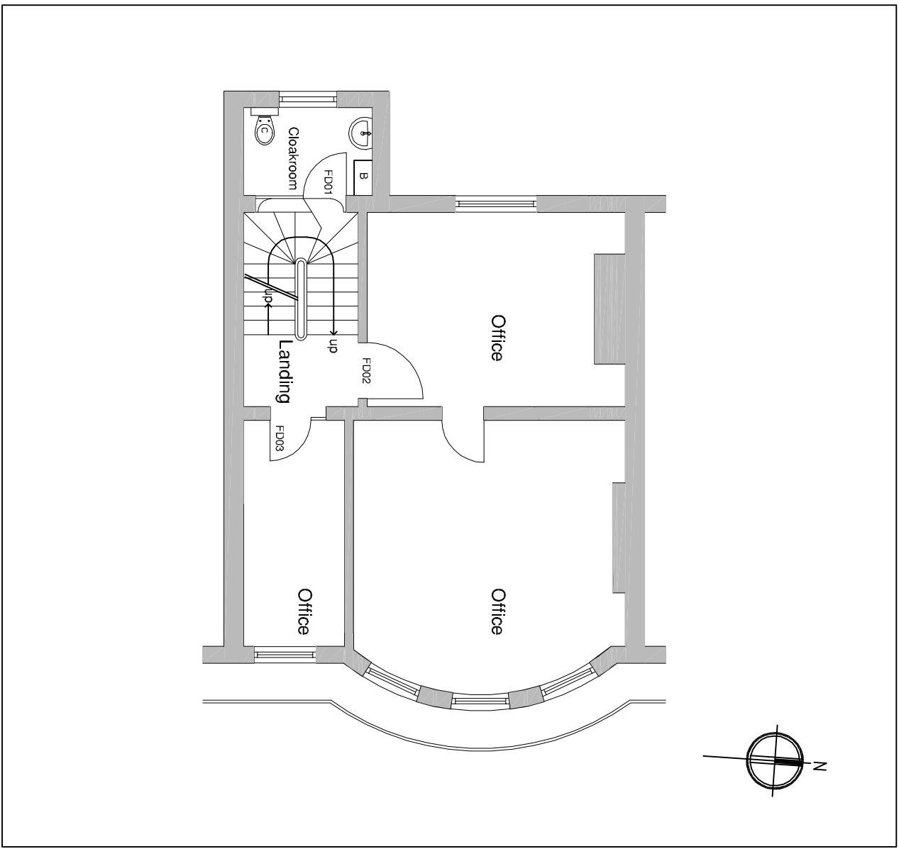
1:100 First Floor Plan as existing
