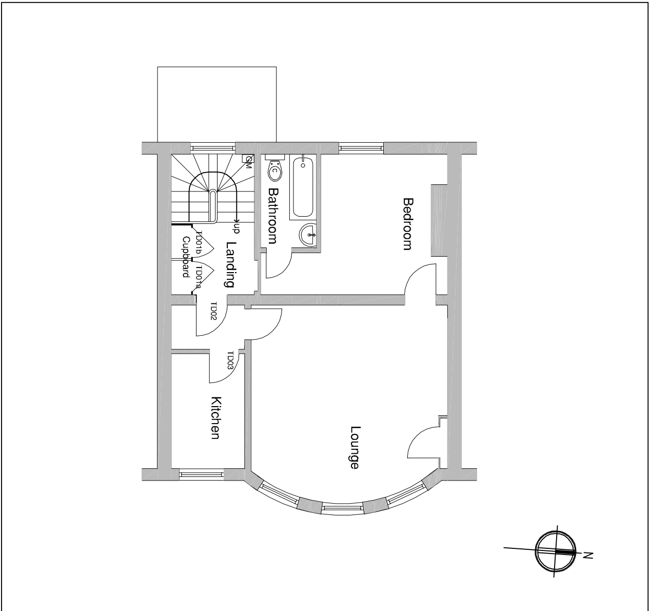
1:100 Third Floor Plan as existing
