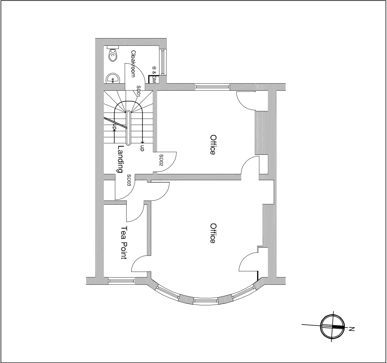
1:100 Second Floor Plan as existing
