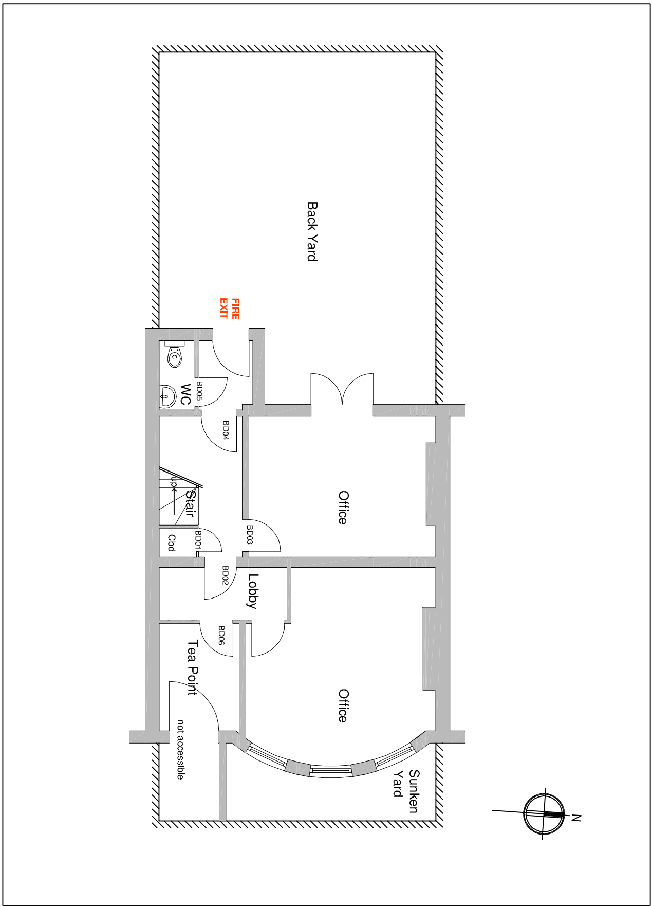
1:100 Basement Plan as existing
