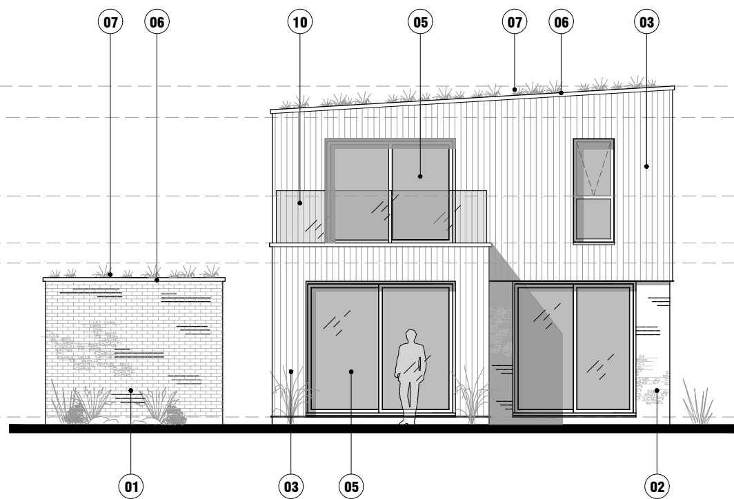
05-Rear Elevation 1:100 Proposed Elevations
