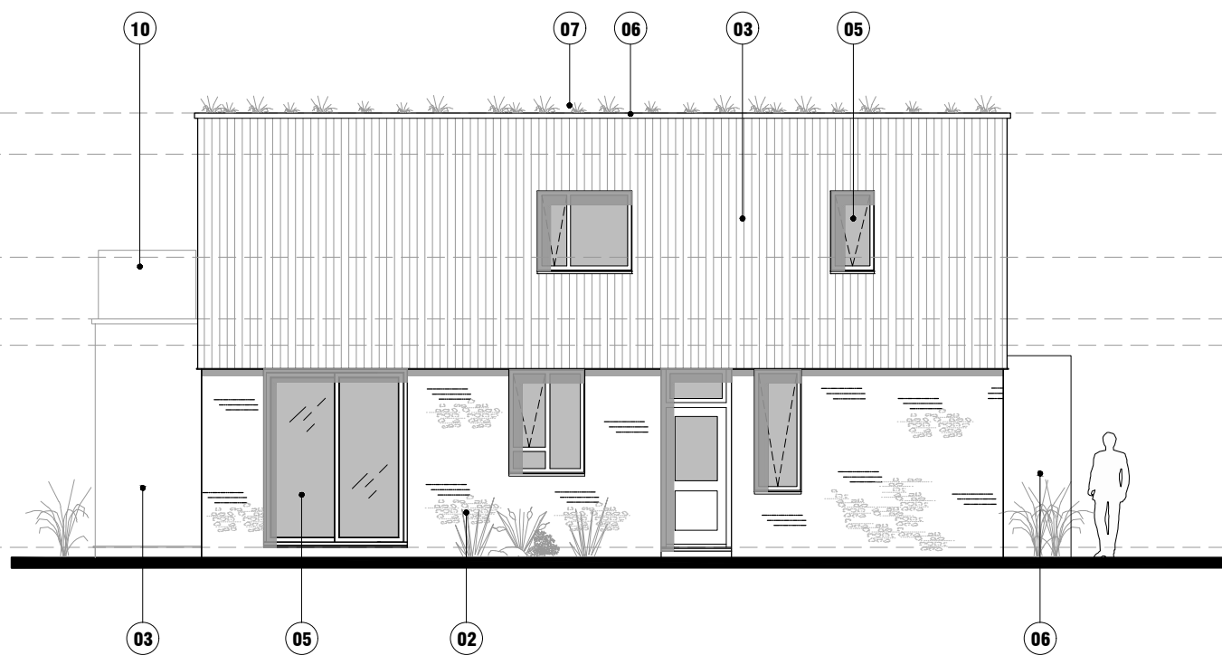
07-Side Elevation 1:100 Proposed Elevations
