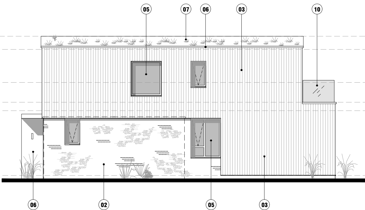
06-SideElevation 1:100 Proposed Elevations
