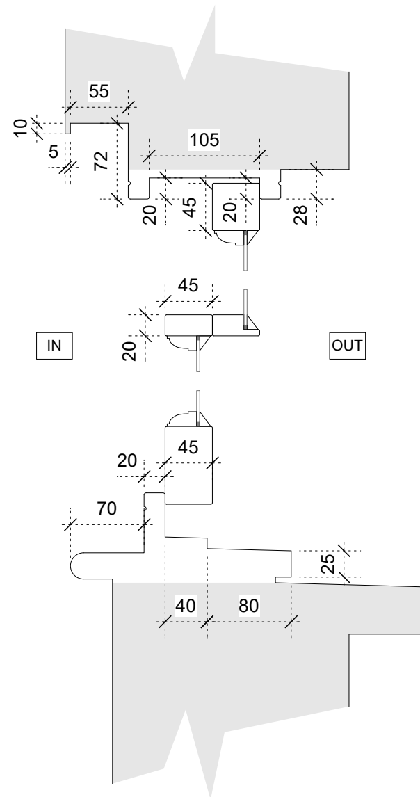
WINDOW TYPE - EW04 TIMBER SASH PUTTY EXTERNALLY VERTICAL SECTION 1:5 @ A3
