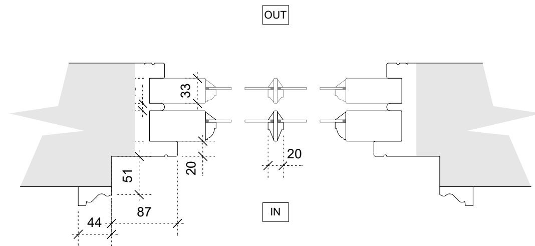
WINDOW TYPE - EW04 TIMBER SASH PUTTY EXTERNALLY HORIZONTAL SECTION 1:5 @ A3
