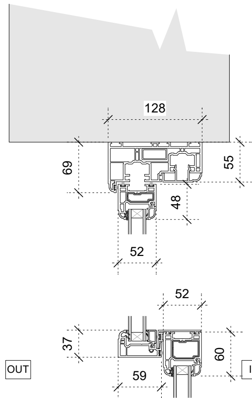
WINDOW TYPE - EW02A uPVC SASH HORIZONTAL SECTION 1:5 @ A3
