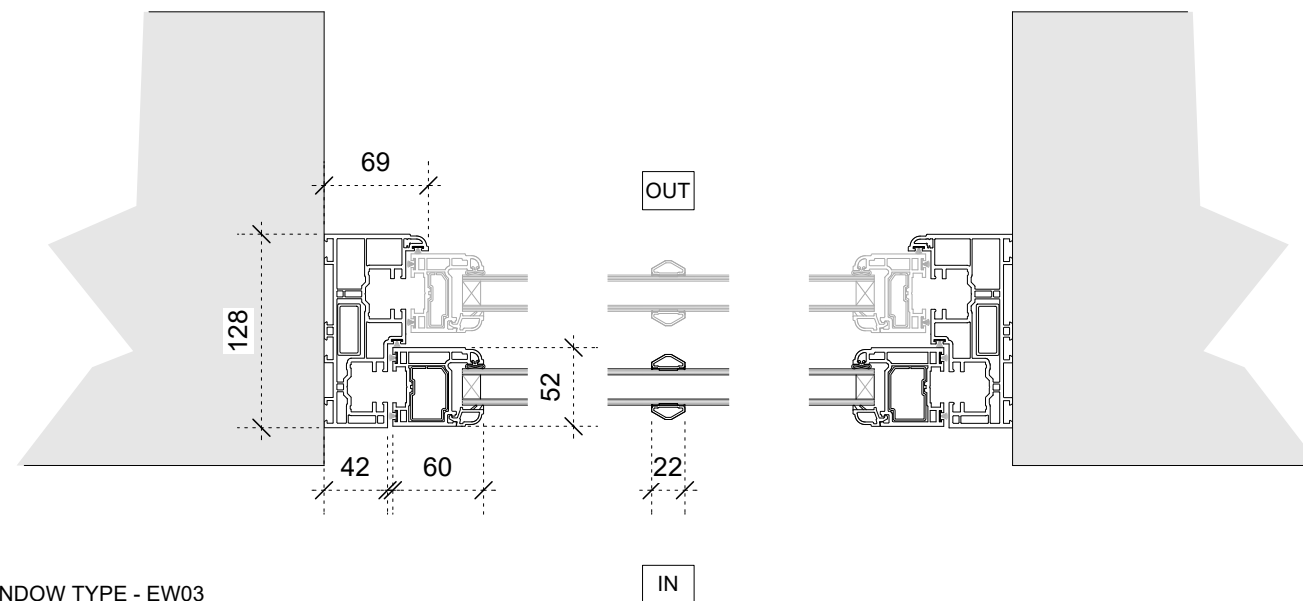
WINDOW TYPE - EW03 uPVC SASH HORIZONTAL SECTION 1:5 @ A3
