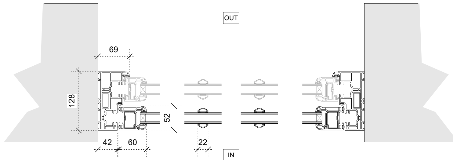
WINDOW TYPE - EW02A uPVC SASH HORIZONTAL SECTION 1:5 @ A3
