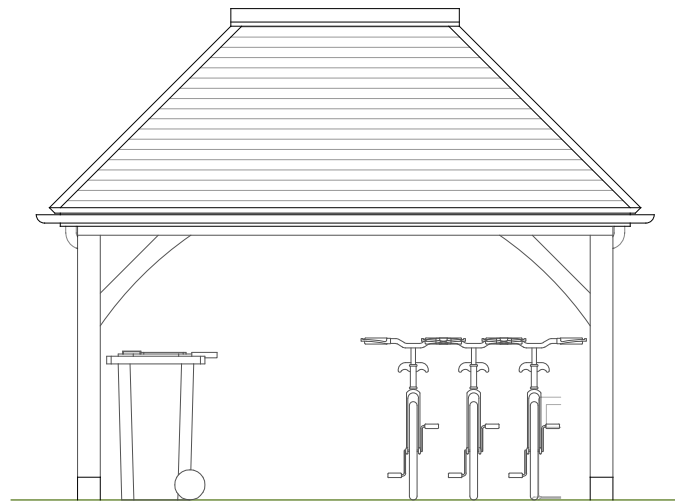
South 1:50 PROPOSED
