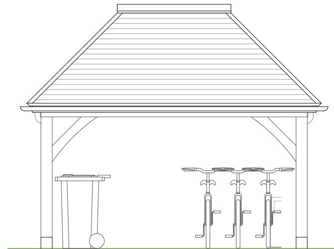
North 1:50 PROPOSED
