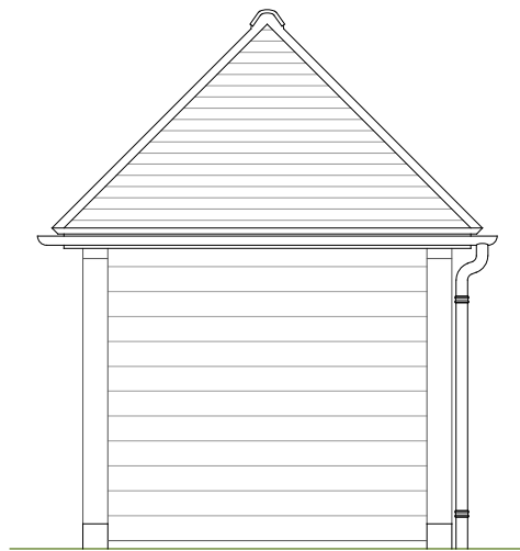
East 1:50 PROPOSED
