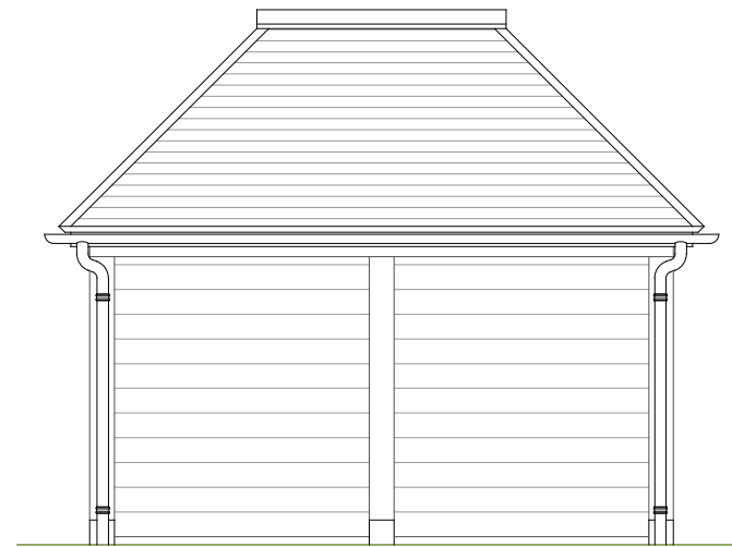
South 1:50 PROPOSED
