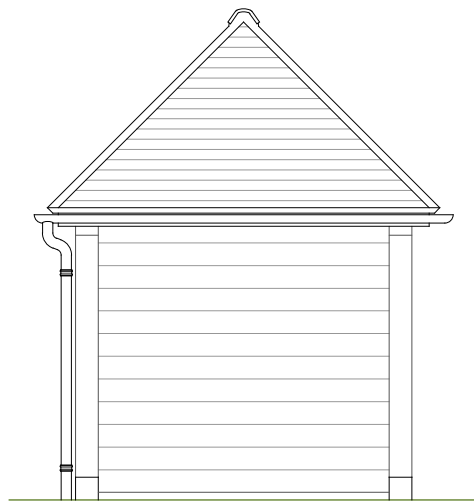
West 1:50 PROPOSED
