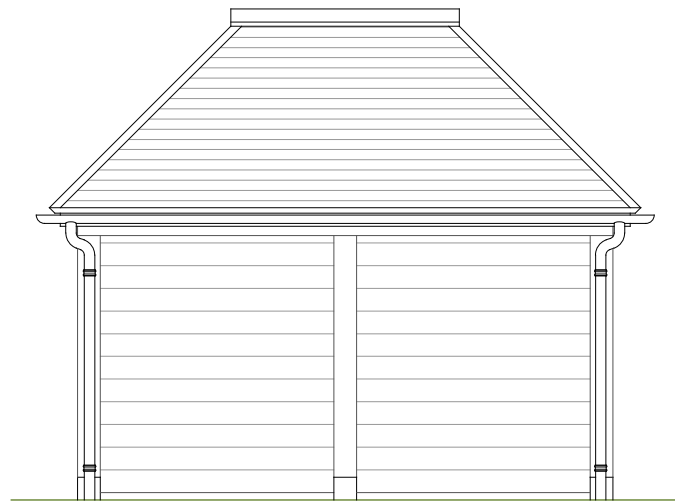
North 1:50 PROPOSED
