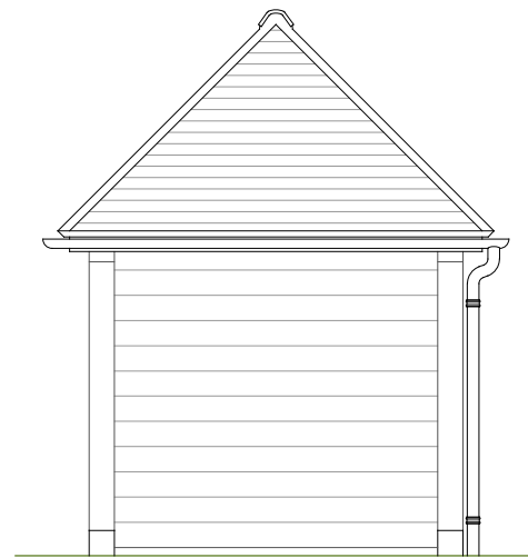
West 1:50 PROPOSED
