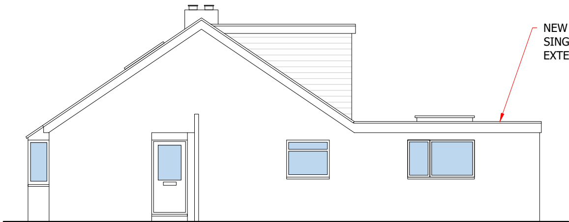
PROPOSED SIDE ELEVATION (N) 1:100
