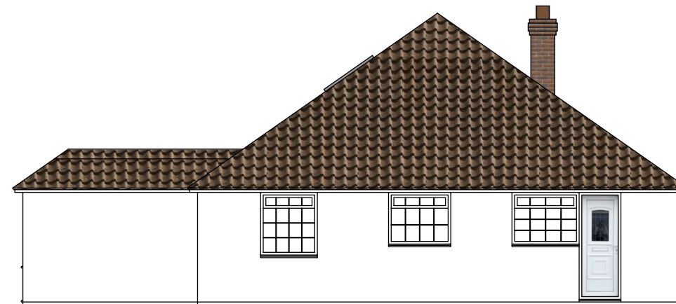
NORTH ELEVATION
