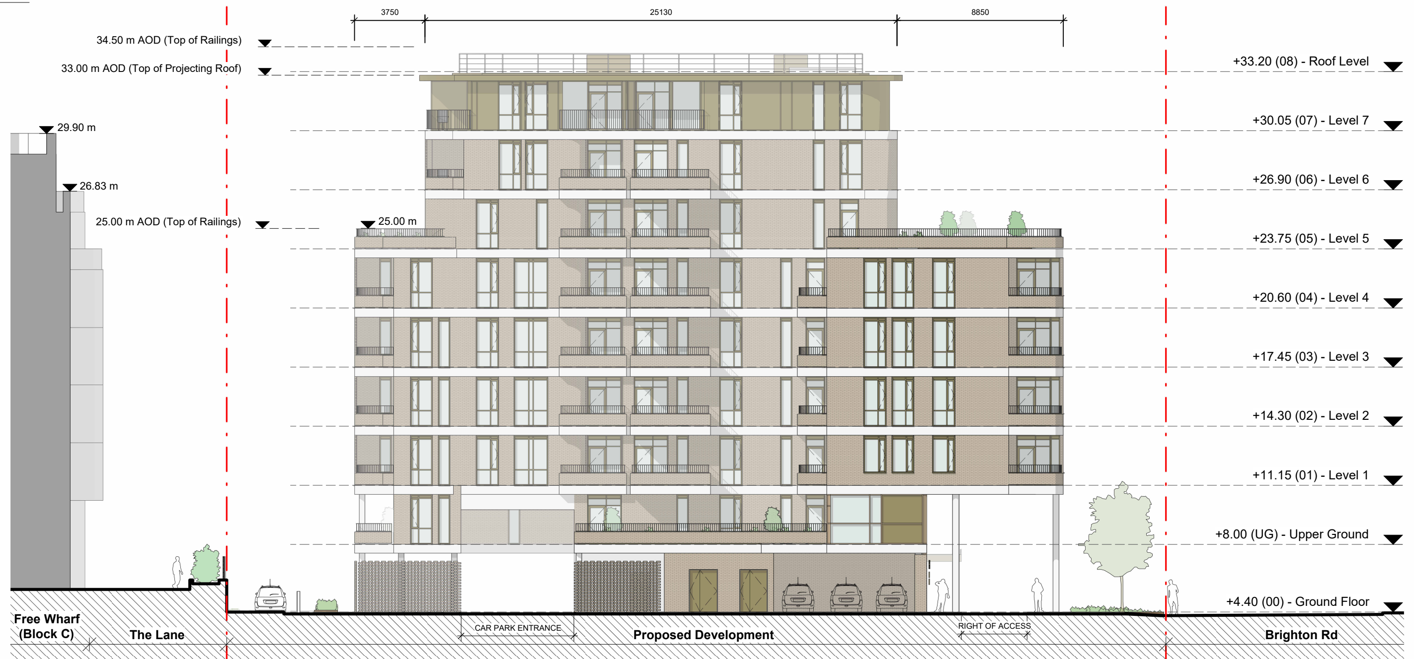
1 Proposed East Elevation 1 : 200
