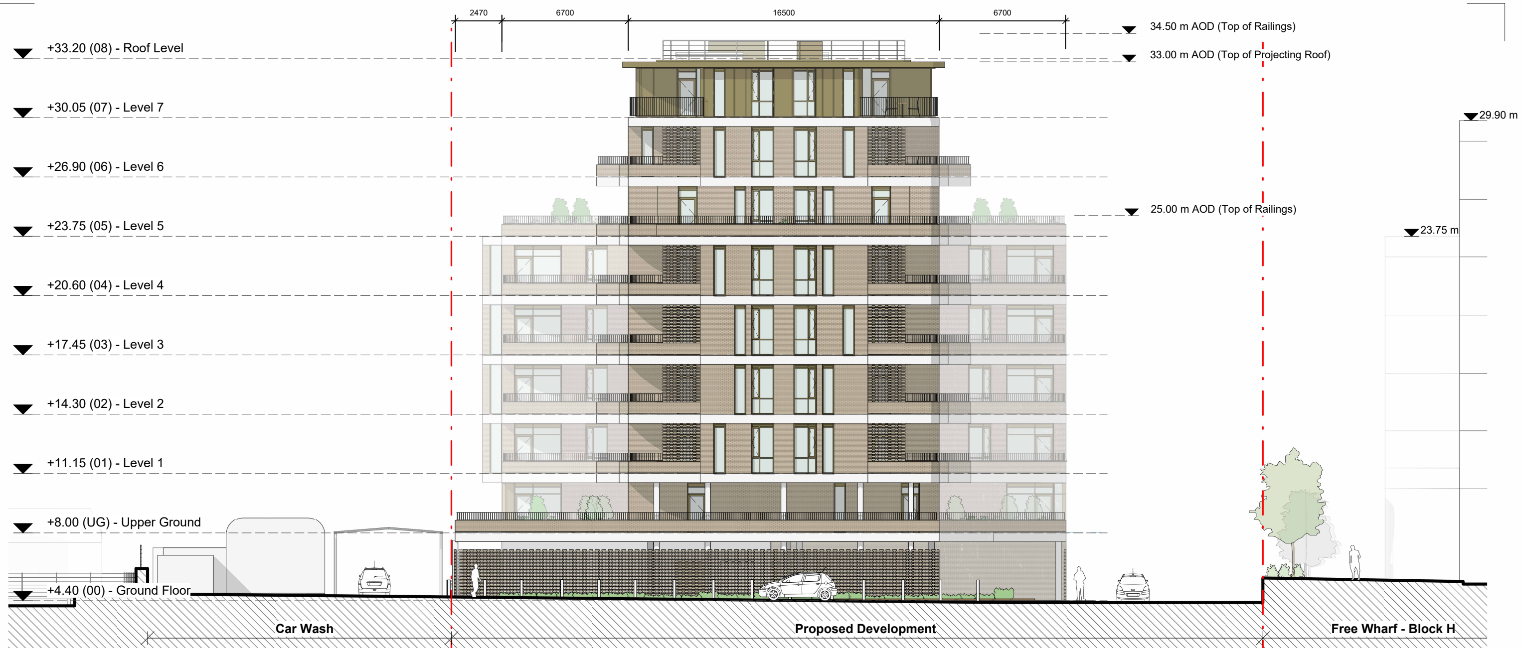
1 Proposed South Elevation 1 : 200
