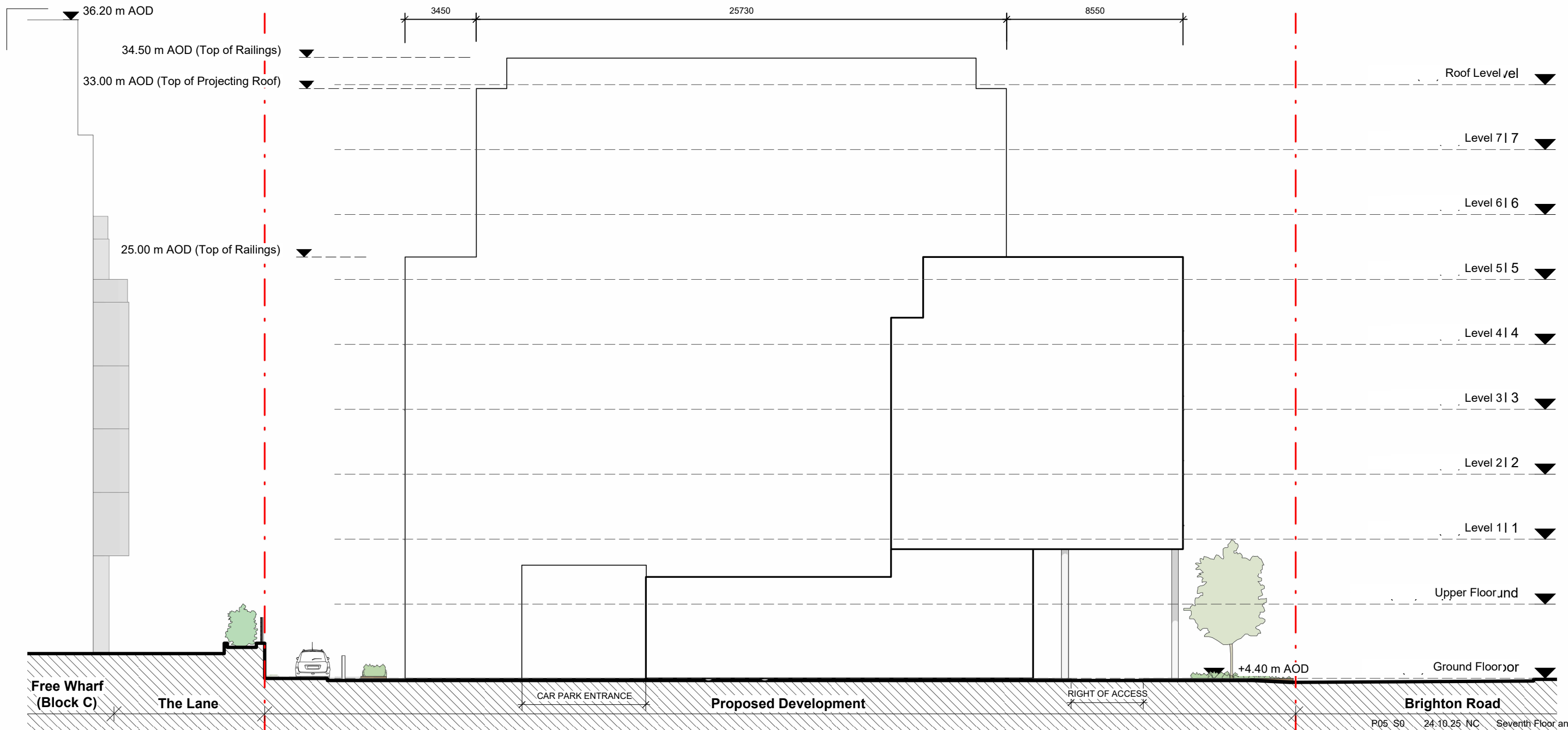
1 Proposed East Elevation 1 : 200
