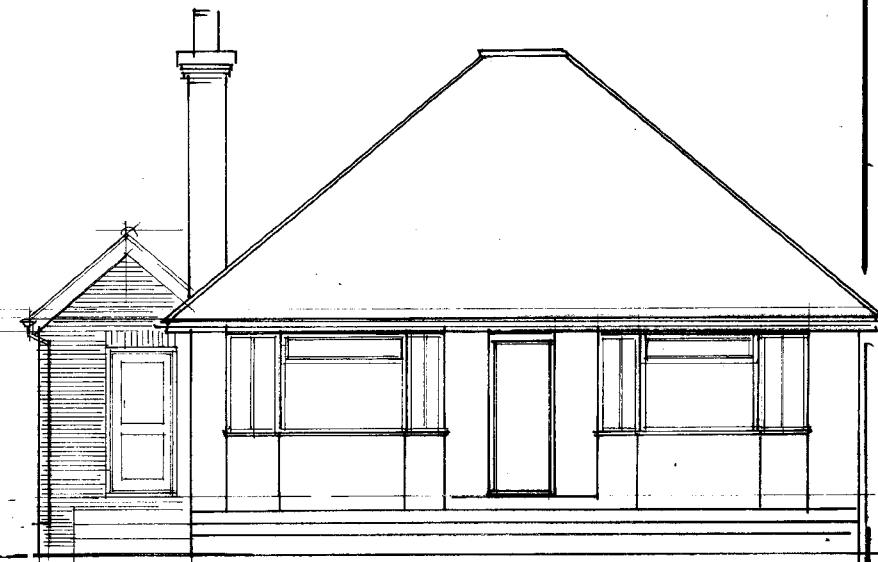
REAR ELEVATION (S)
