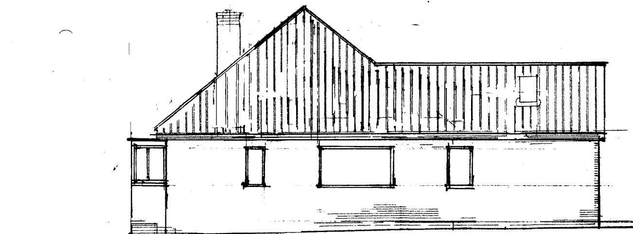
EAST ELEVATION
