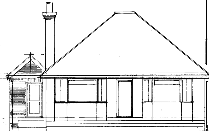
REAR ELEVATION (S)
