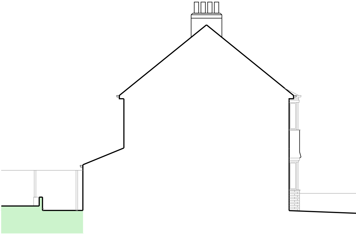
Southern Elevation
