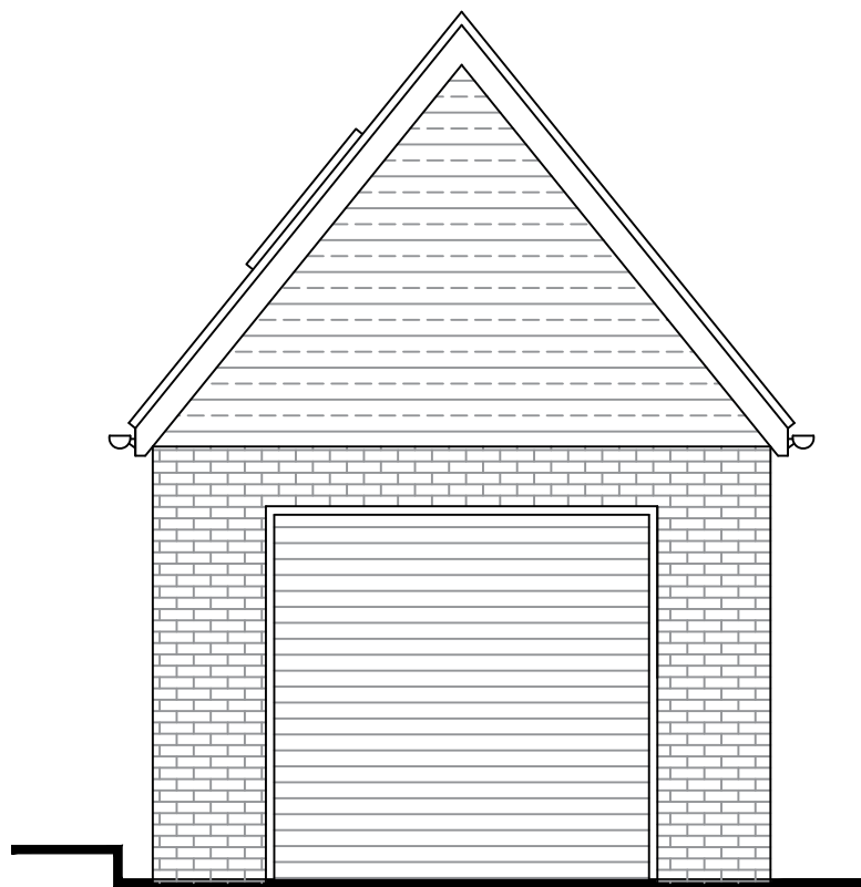
Proposed Front (East) Elevation (Scale 1:50)
