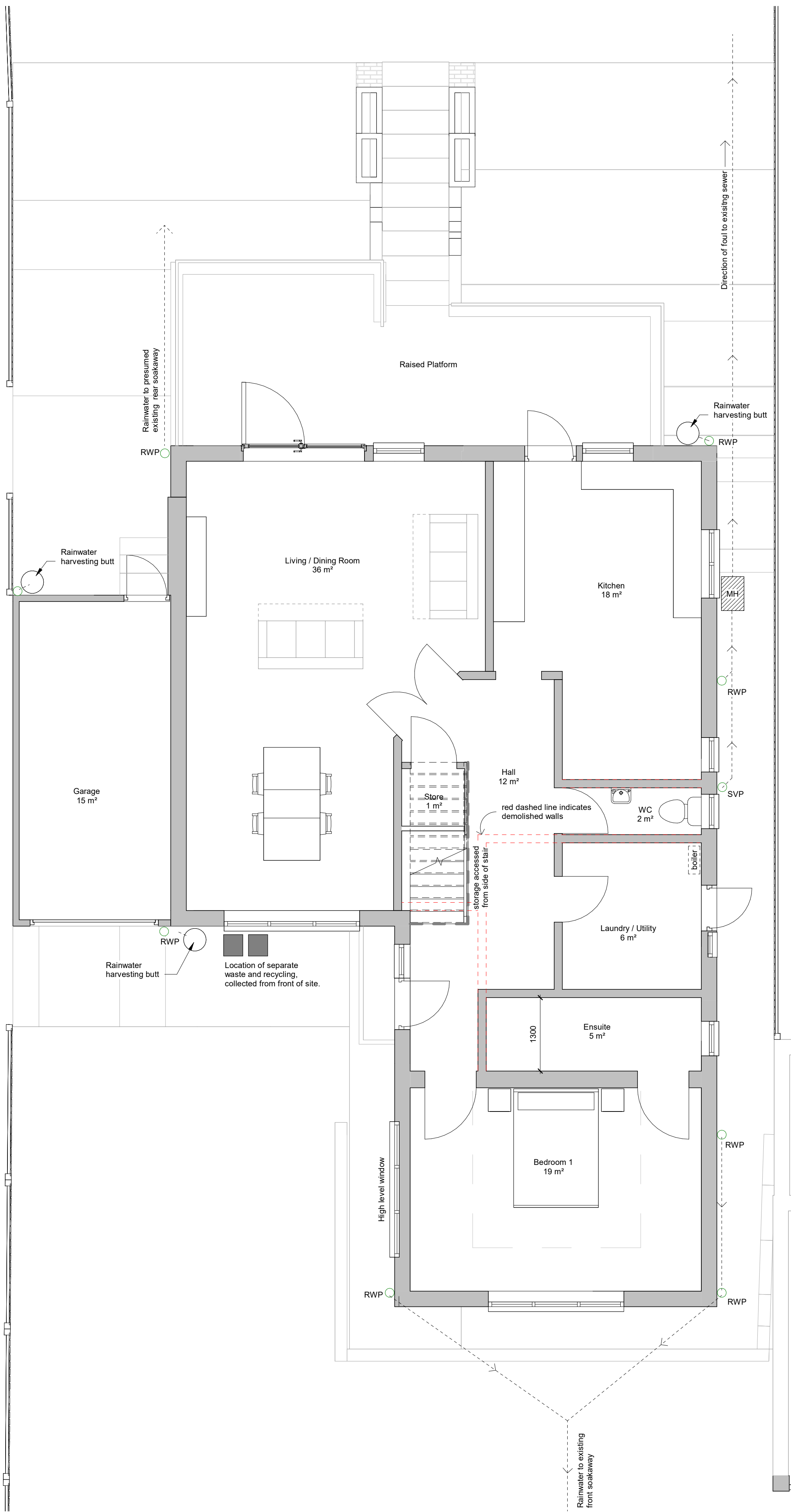
1 Proposed Ground FFL 1 : 50
