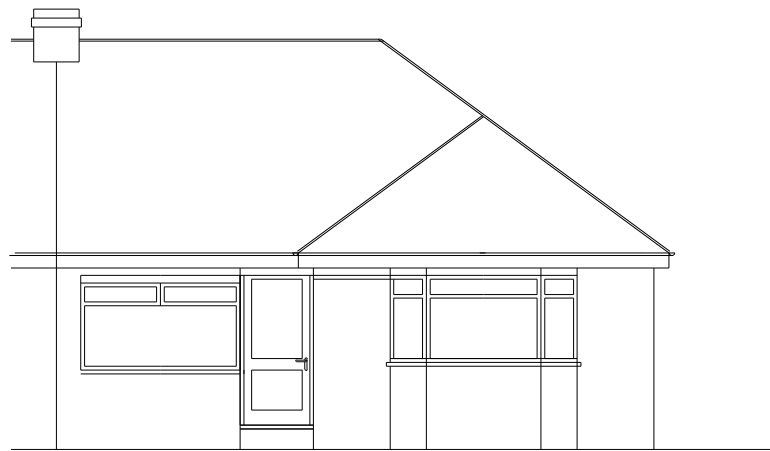
Existing - West elevation
