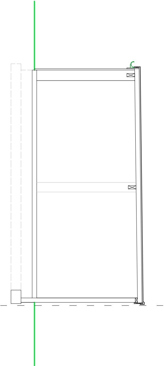
EXISTING CROSS SECTION 'AA'
