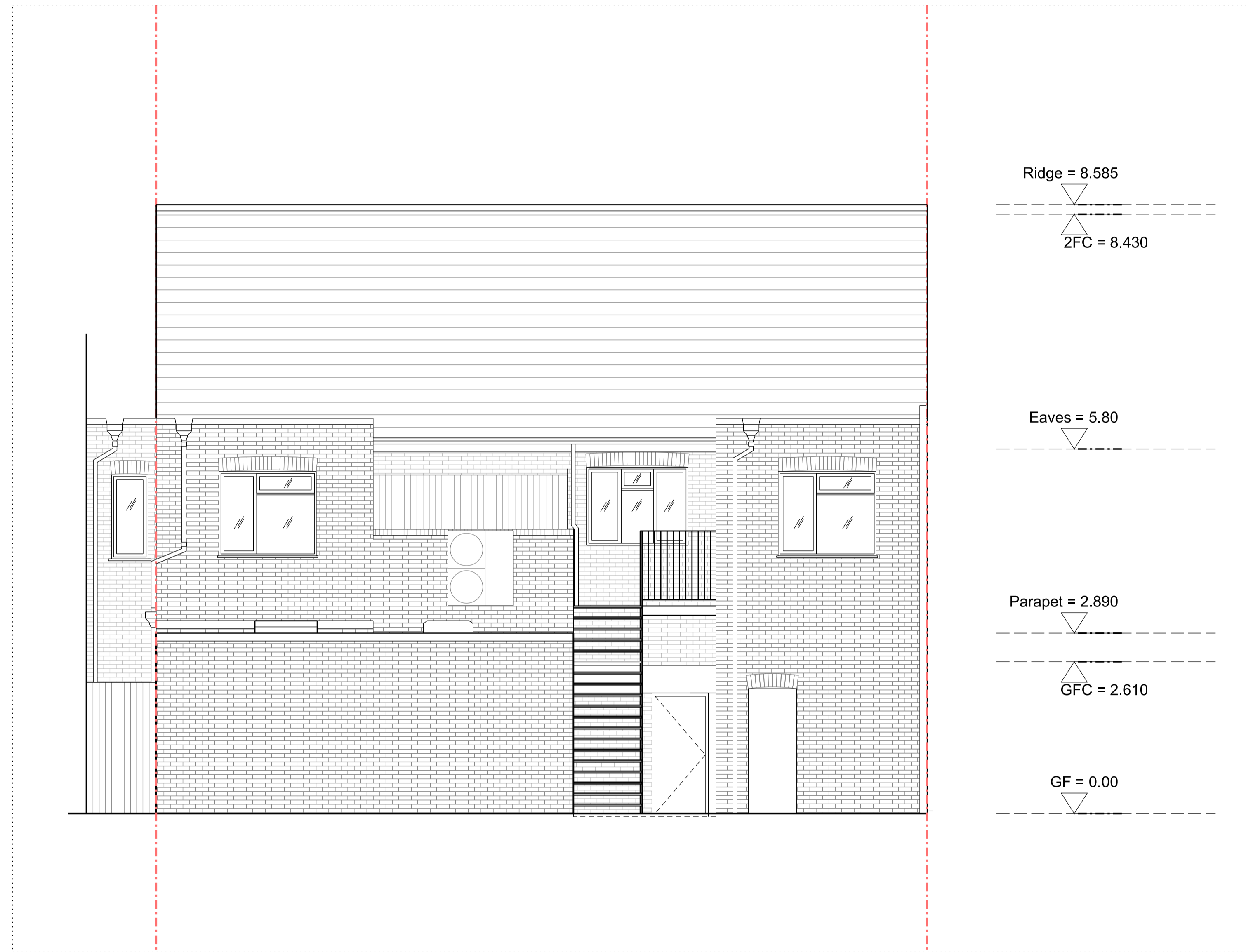
Existing South-West Elevation
