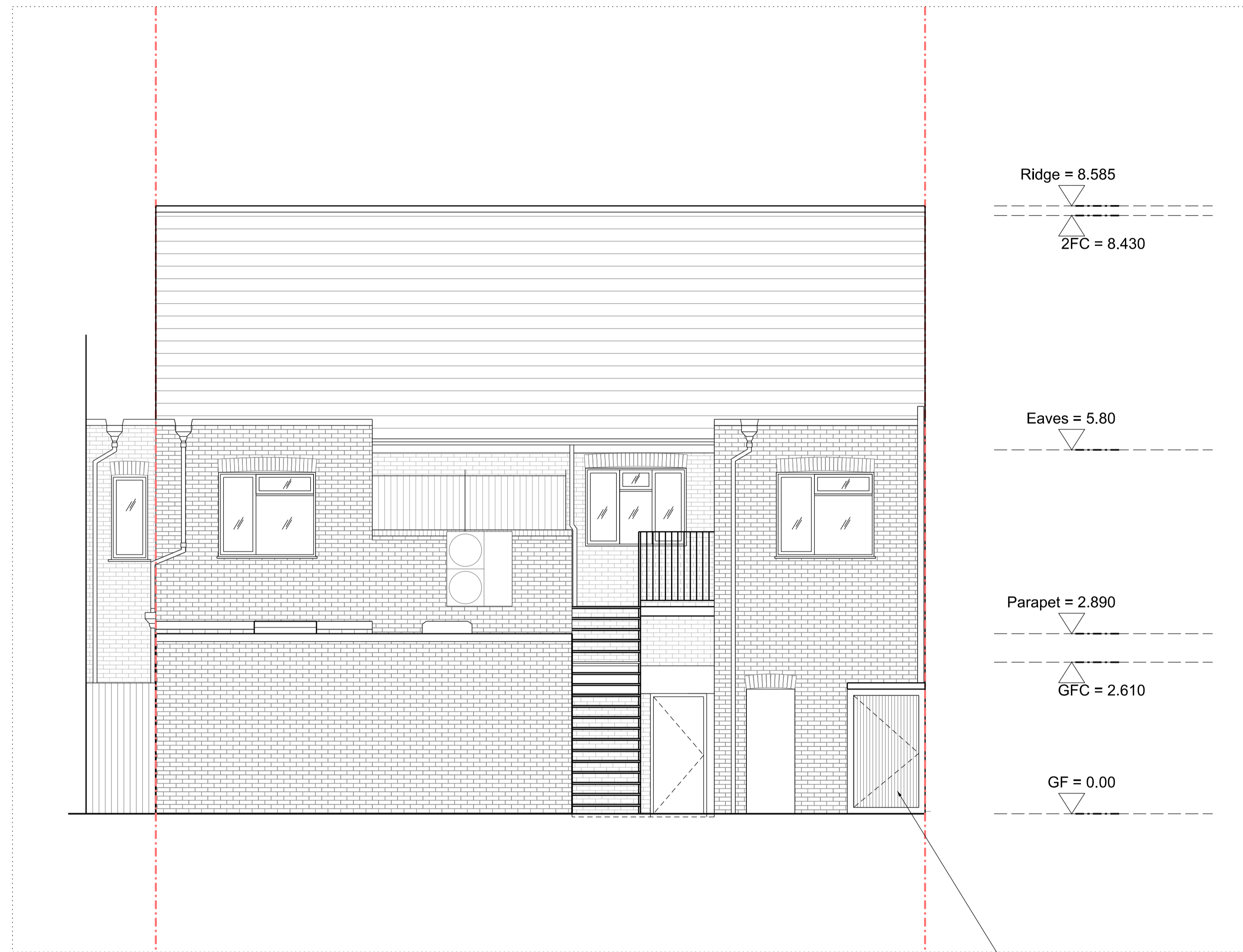
Proposed South-West Elevation
