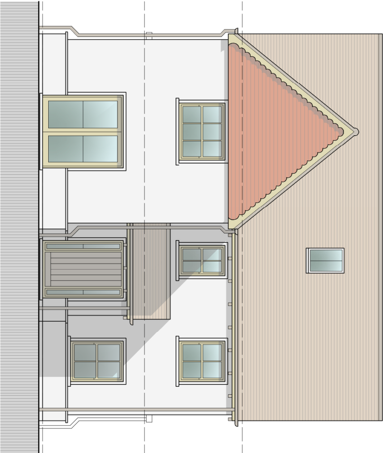
UNIT R7 Proposed front / south elevation Scale 1:100@A3
