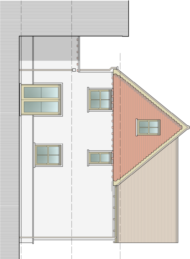
UNIT R7 Proposed side / west elevation Scale 1:100@A3
