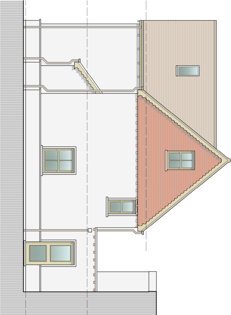
UNIT R7 Proposed side / east elevation Scale 1:100@A3
