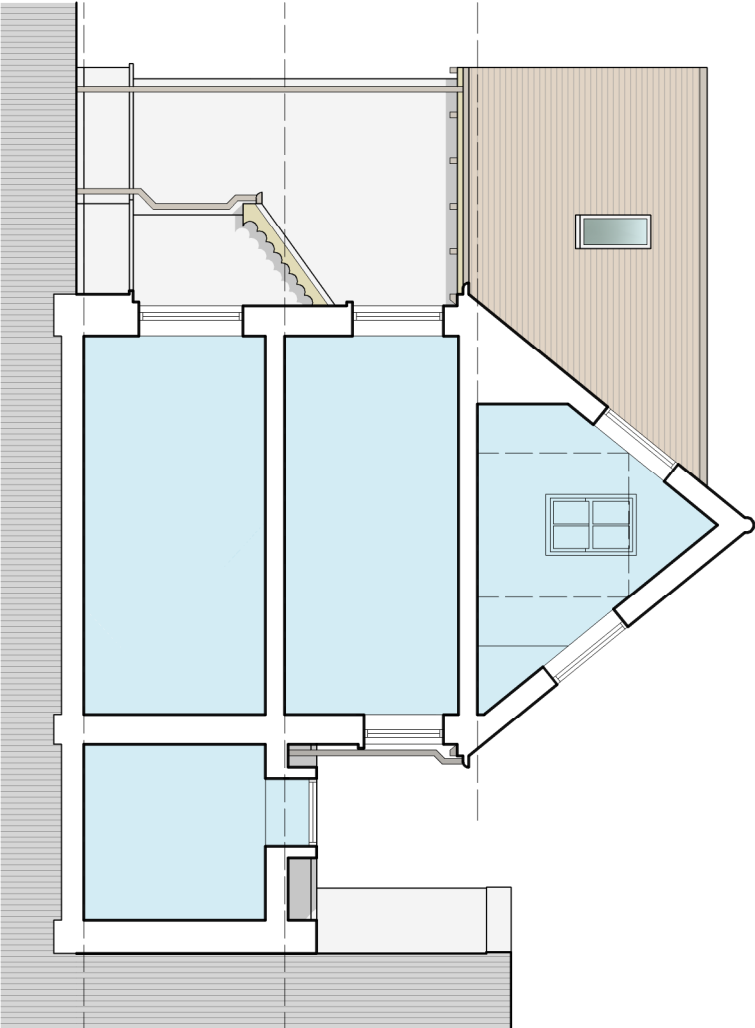
UNIT R7 Proposed section Scale 1:100@A3
