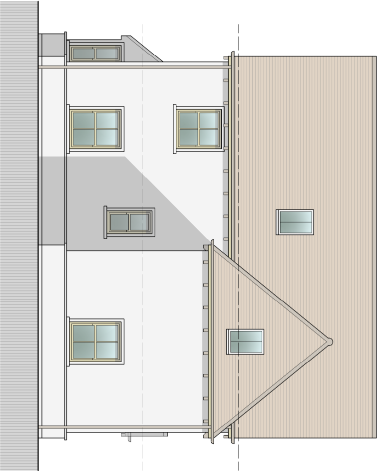
UNIT R8 Proposed rear / north elevation Scale 1:100@A3
