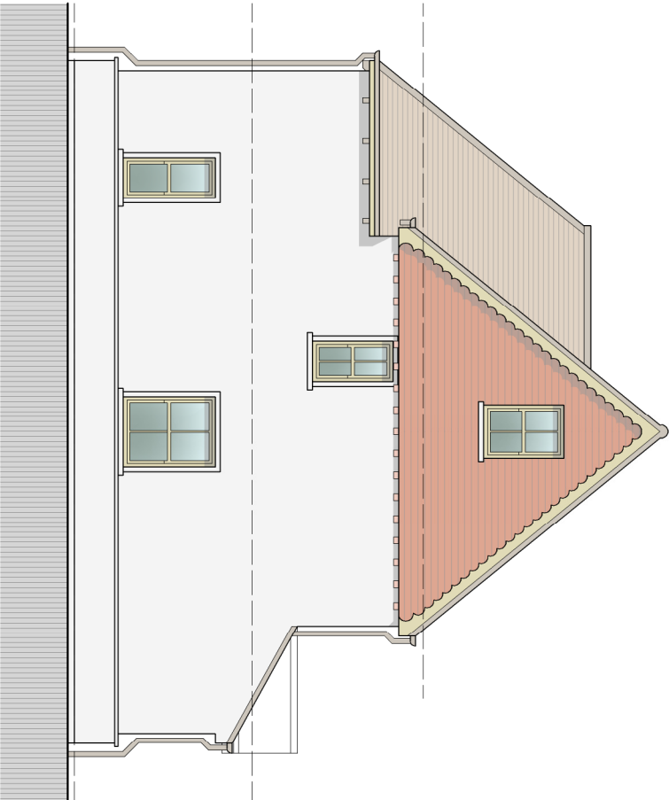
UNIT R8 Proposed side / west elevation Scale 1:100@A3
