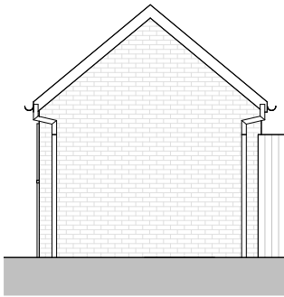
Garage - East Elevation 1 : 100
