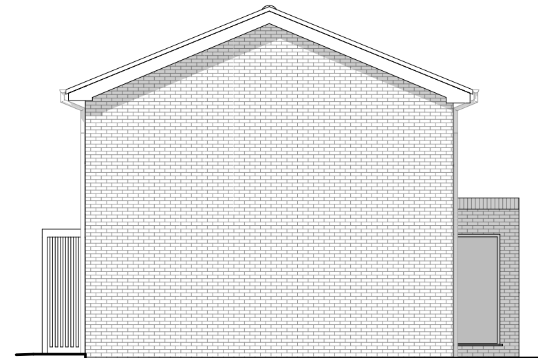
Proposed Side Elevation (South) Scale 1:100 @ A3
