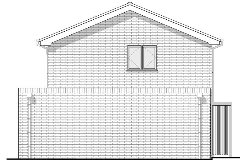
Proposed Side Elevation (North) Scale 1:100 @ A3
