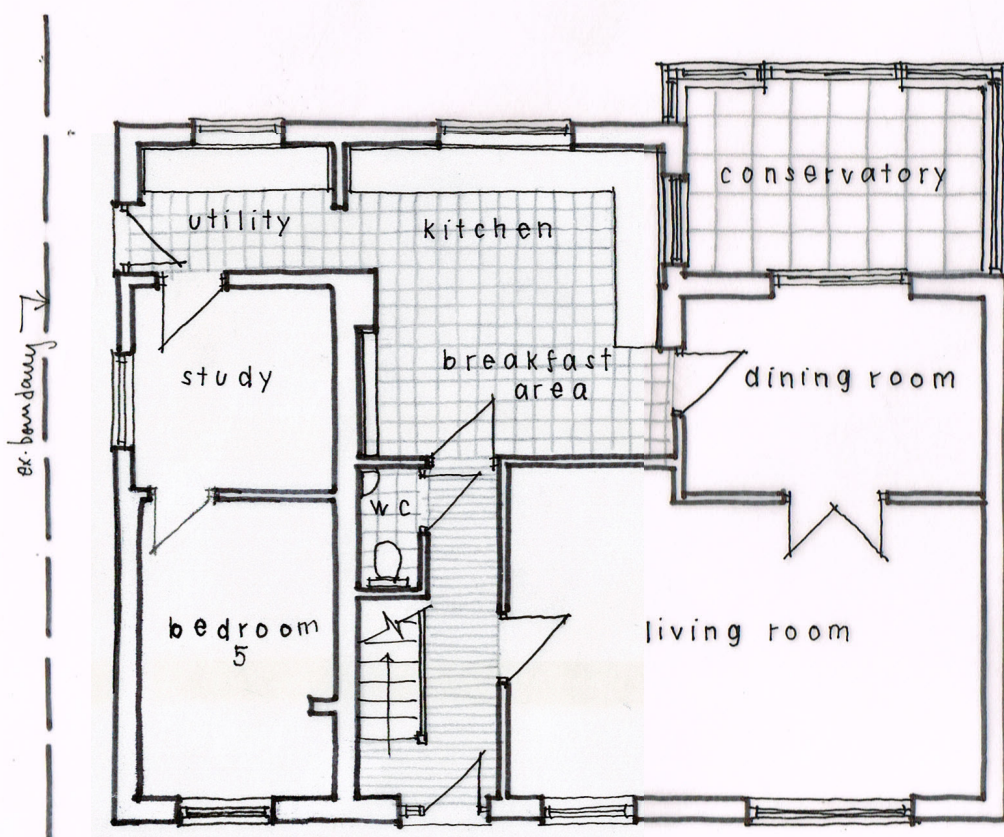
GROUND FLOOR PLAN 1:100 @ A3
