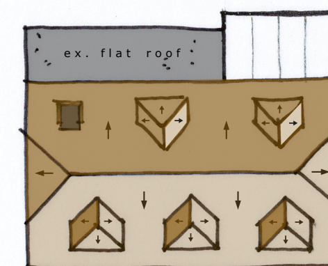
ROOF PLAN 1:200
