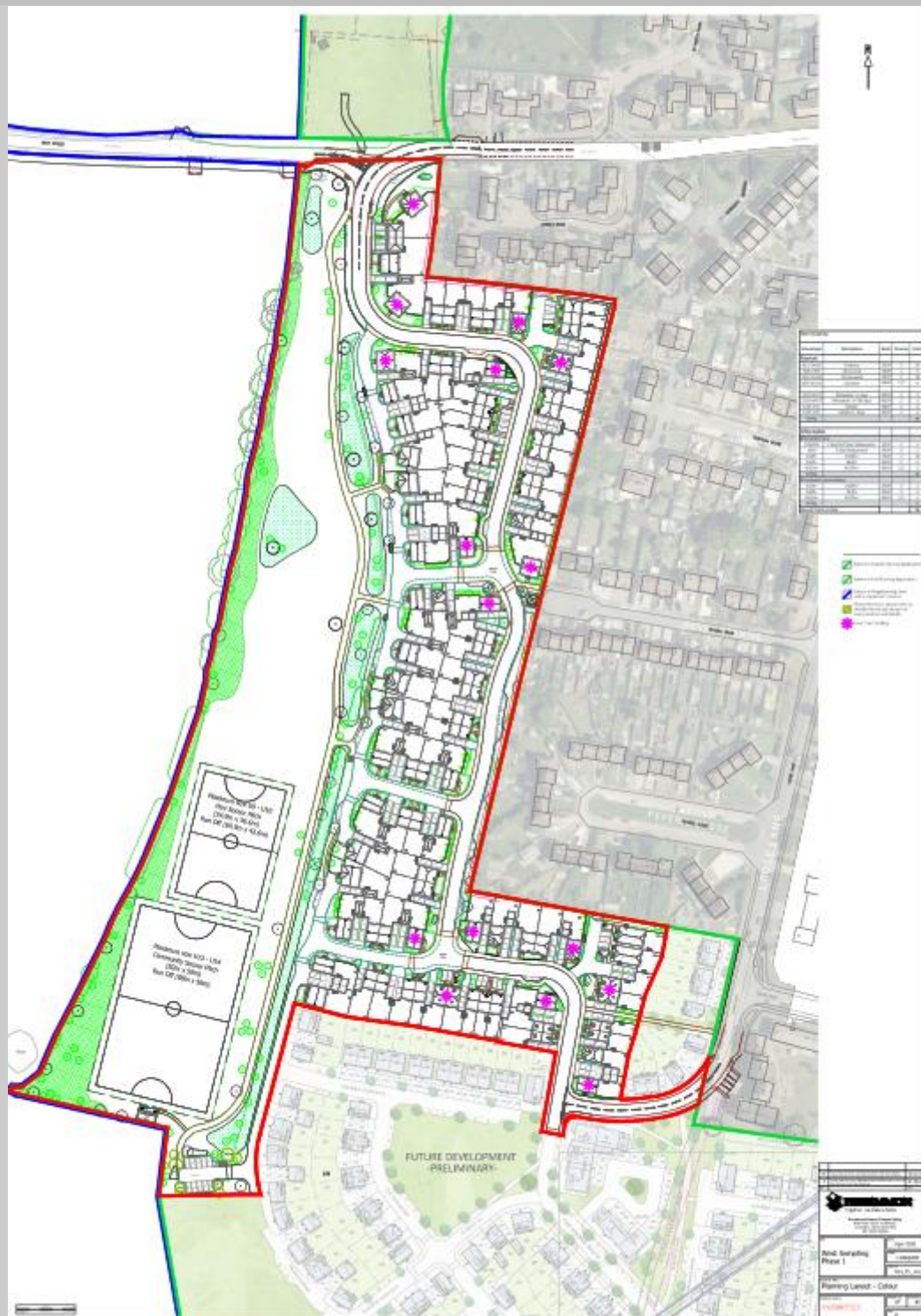
Site Layout
