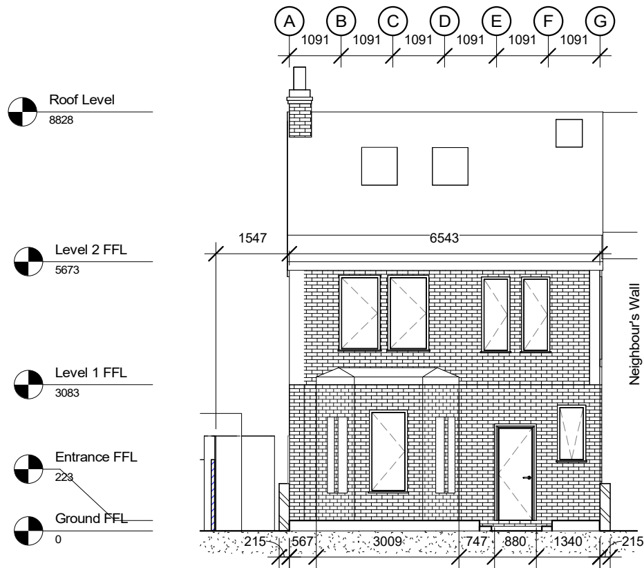
Planning - South Elevation - Existing 1 : 100
