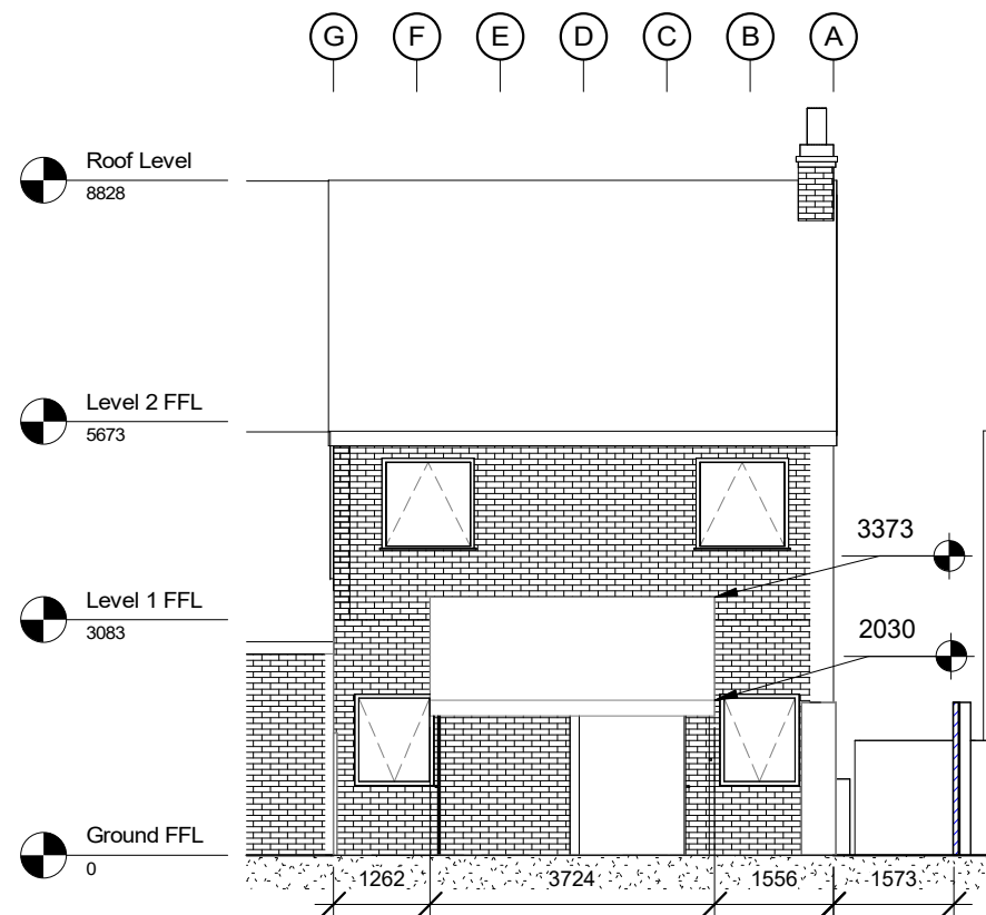
Planning - North Elevation - Existing 1 : 100
