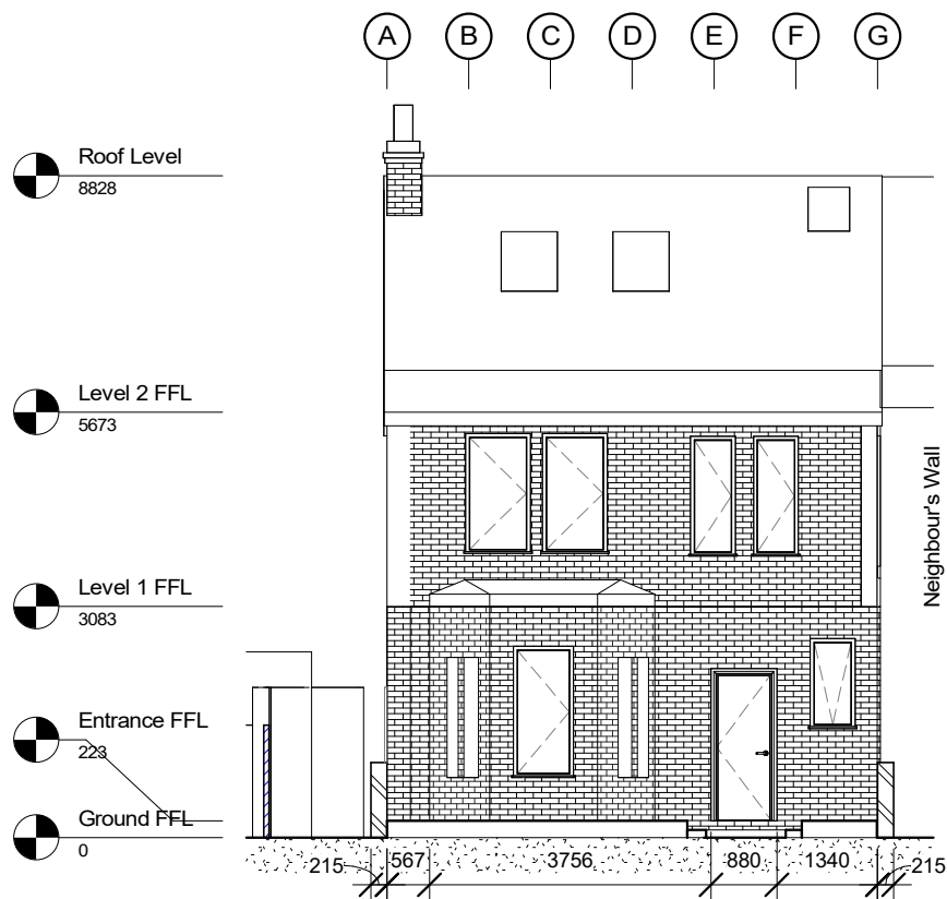
Planning - South Elevation - Proposed 1 : 100
