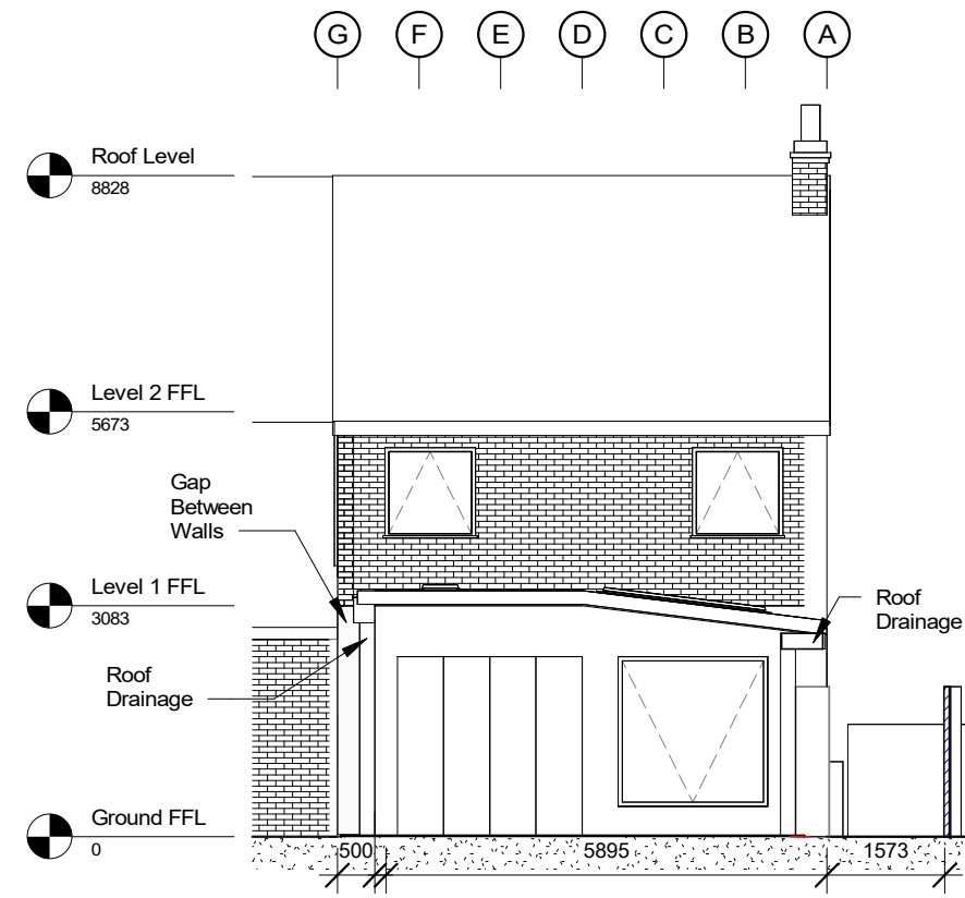
Planning - North Elevation - Proposed 1 : 100
