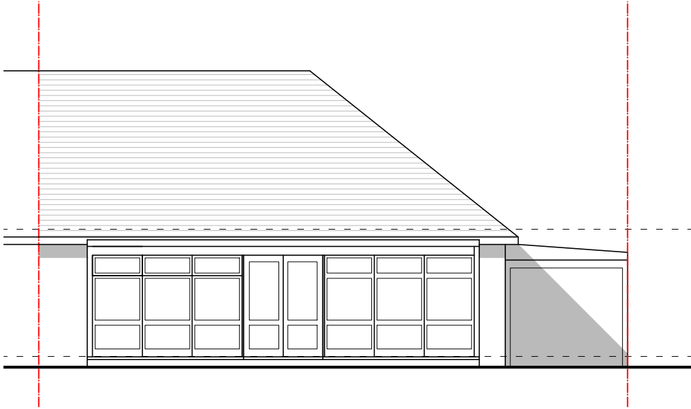
01 SOUTH ELEVATION S.02 AS EXISTING_1:100 @ A3
