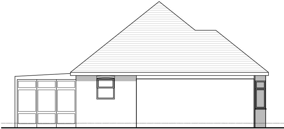
02 EAST ELEVATION S.02 AS EXISTING_1:100 @ A3
