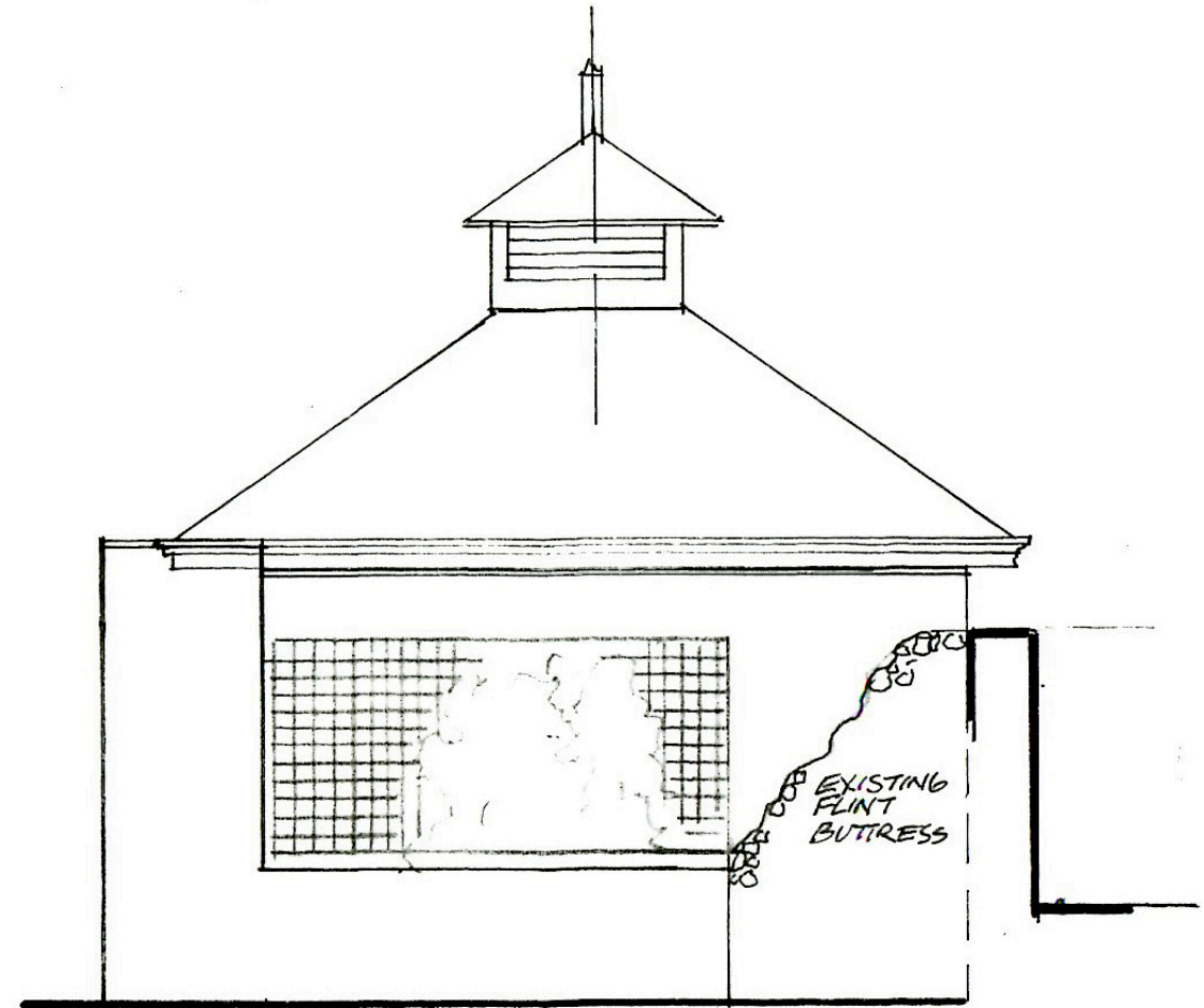
North Elevation
