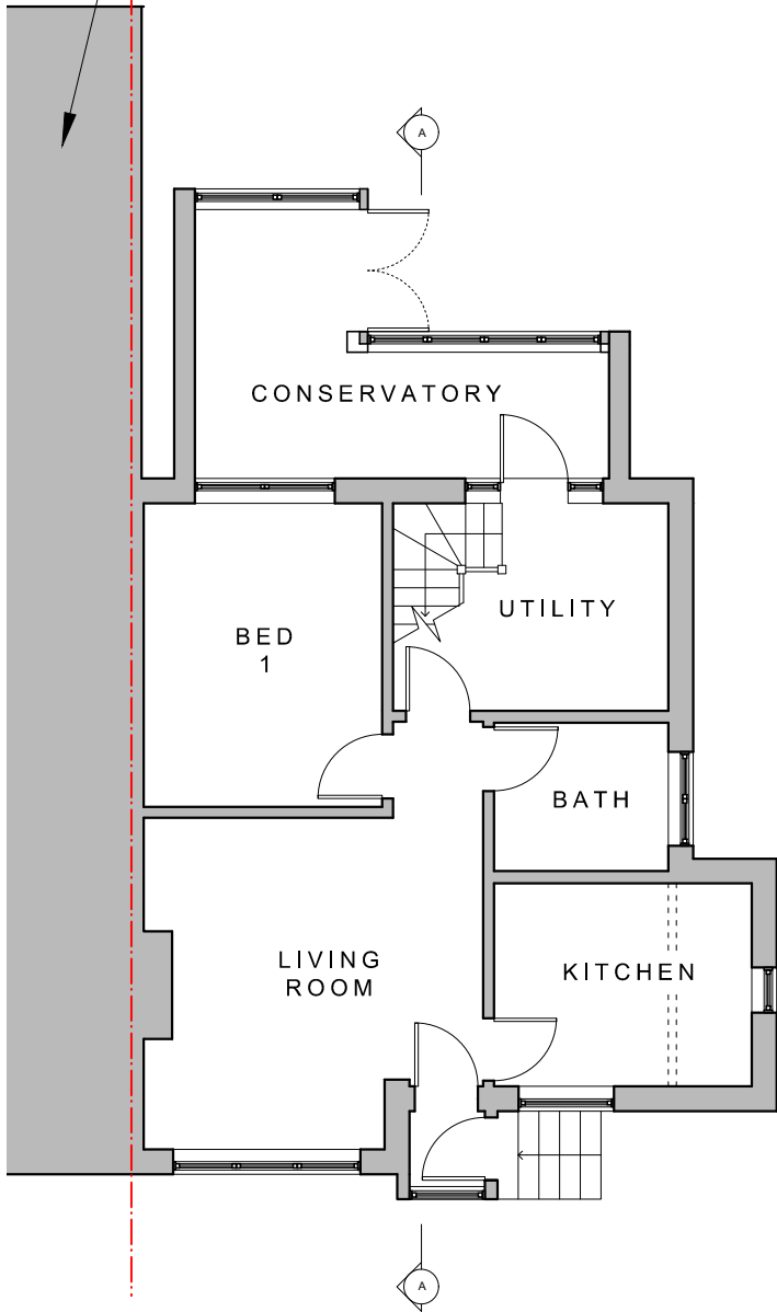
01 GROUND FLOOR PLAN S.01 AS EXISTING_1:100 @ A3
