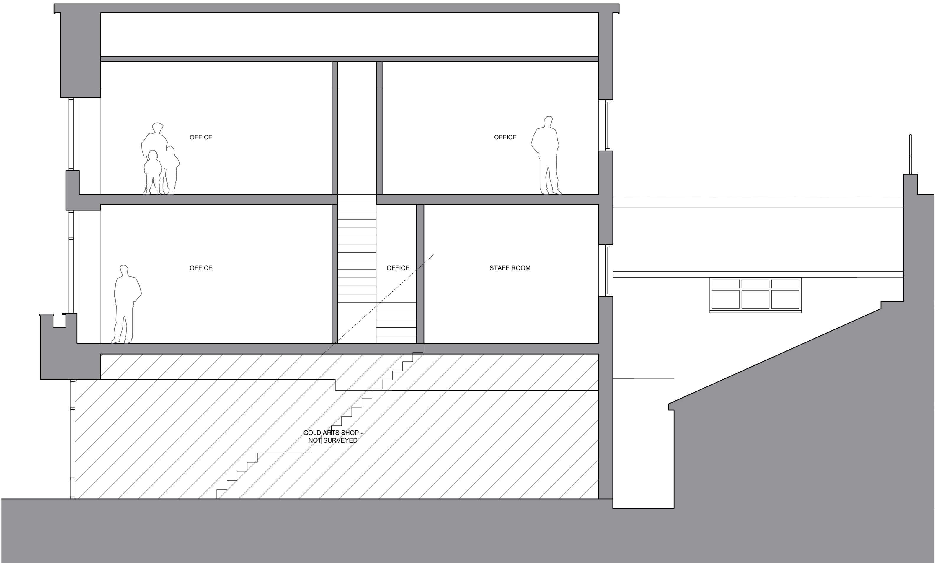
Section A-A @ 1:50 - NO CHANGE
