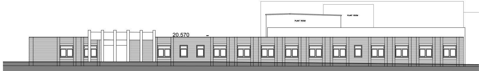
Elevation North
