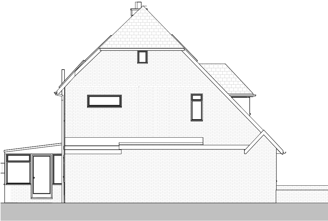
Existing South Elevation
