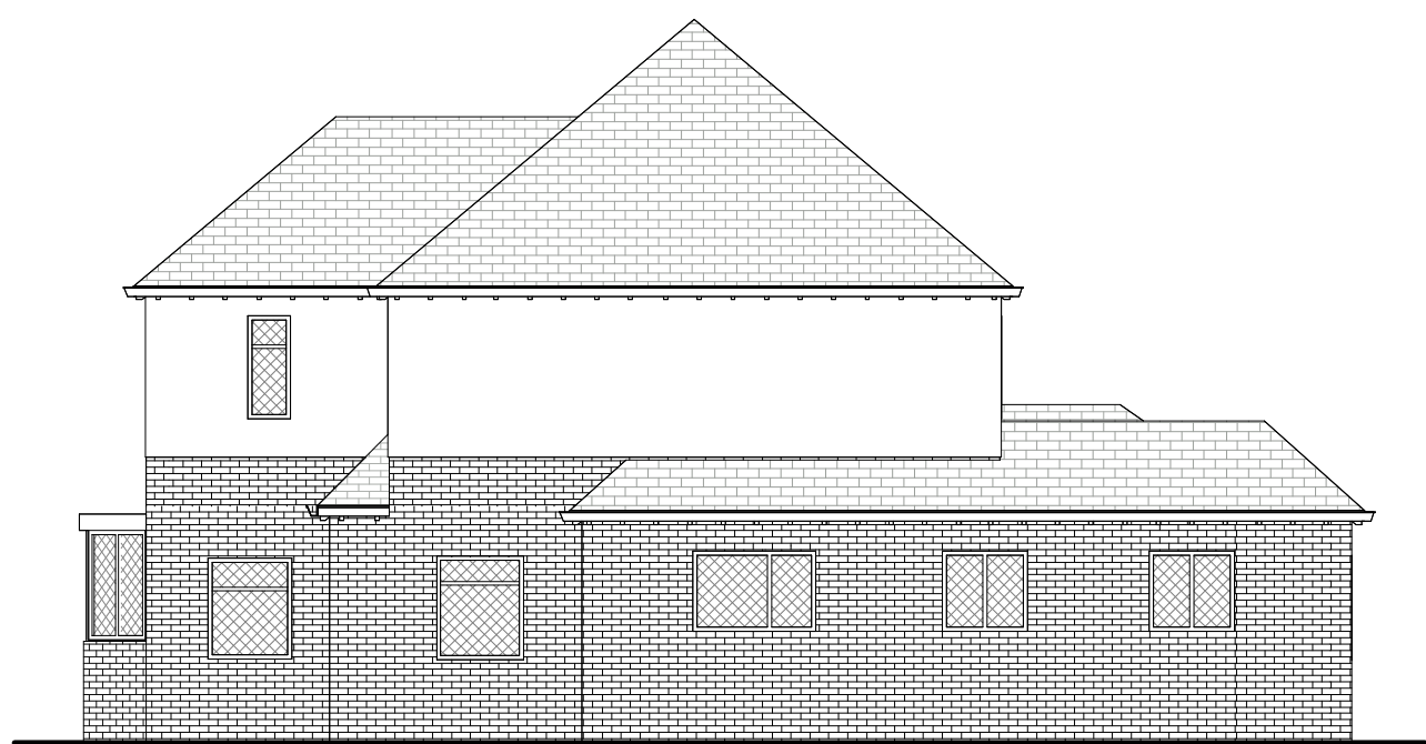
Existing South Elevation 1 : 100
