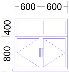
1200 X 1200 28mm QS Bead Drainage: BASE
