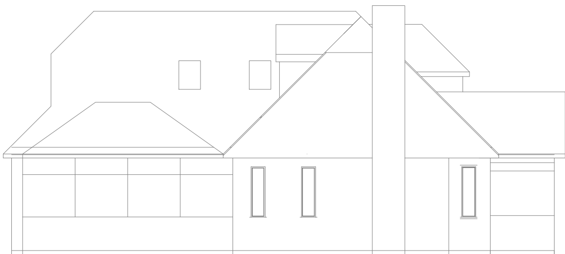
EXISTING SIDE ELEVATION facing west
