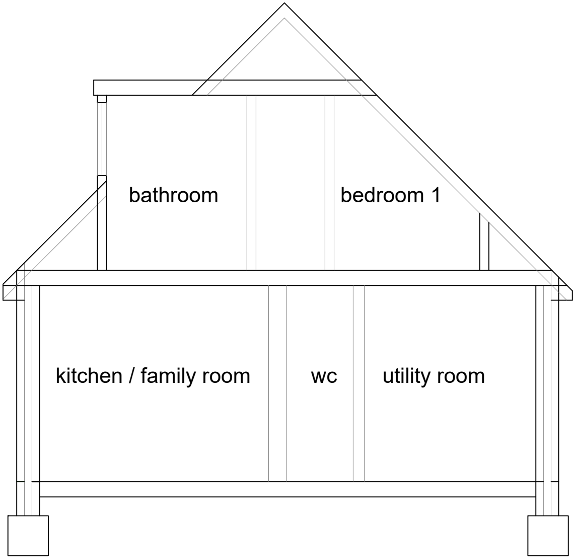
PROPOSED SECTION
