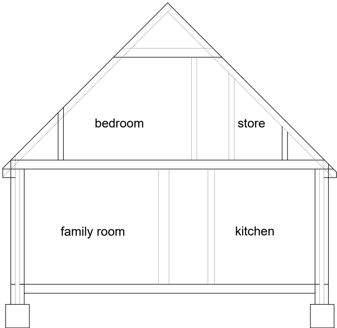
EXISTING TYPICAL SECTION
