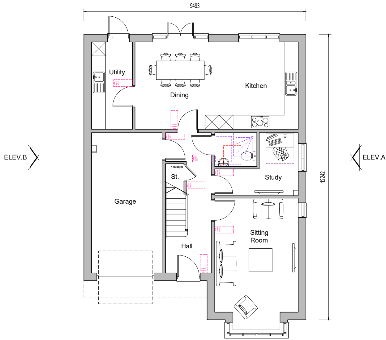
Ground Floor Plan Plot 462
